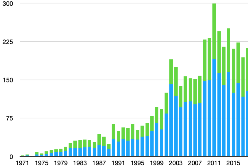
Figure 17. The growth of helicity studies in solar physics over my career, measured by the annual number of refereed (blue) and total (green) research publications in the NASA ADS database as of the time of writing whose abstracts contain the words solar and helicity. Contributions to this figure of which I am most proud are: latitude variation of the helicity of photospheric magnetic fields of active regions (Pevtsov, Canfield, and Metcalf, 1995); evidence that magnetic flux emerges already carrying current (Leka et al., 1996); AGU Conference on magnetic helicity in space and laboratory plasmas (Brown, Canfield, and Pevtsov, 1999); relation between sigmoidal morphology and eruptive solar activity (Canfield, Hudson, and McKenzie, 1999); properties of interplanetary magnetic clouds and geomagnetic storms associated with eruptions of coronal sigmoids (Leamon, Canfield, and Pevtsov, 2002); predictions of energy and helicity in large eruptive flares (Kazachenko et al., 2012).
