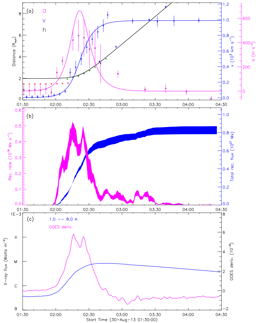
Figure 49: 20130830_STB195_rec_wavelnth.1600_GOES_used
