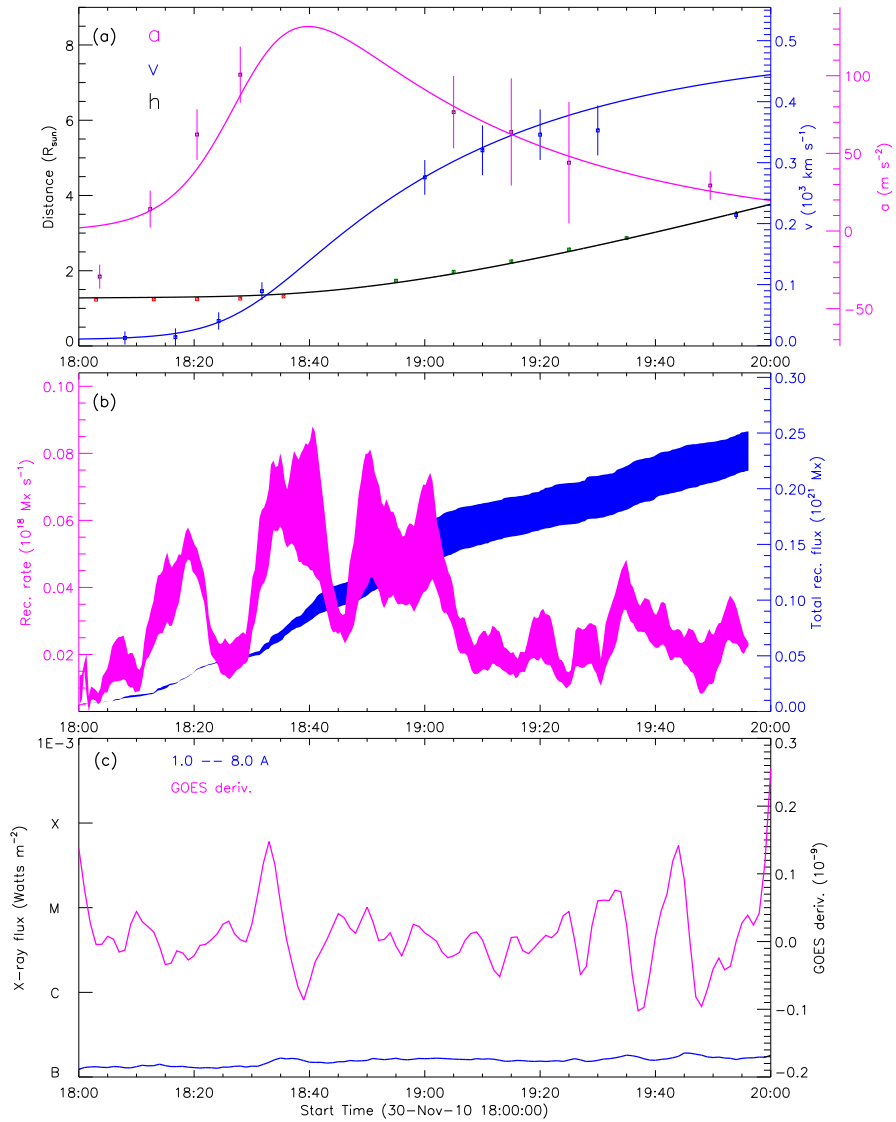
Figure 4: 20101130_18_STA195_rec_wavelnth_304_GOES_not_used
