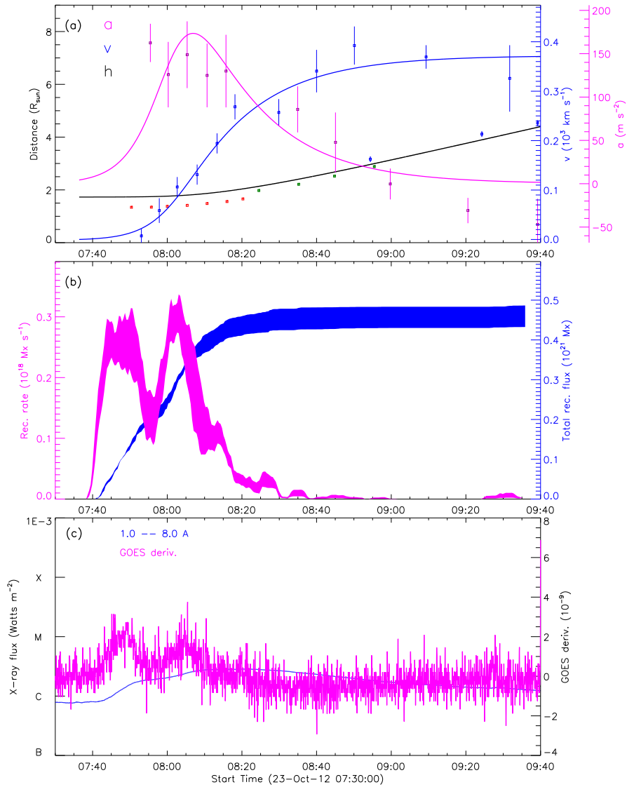
Figure 39: 20121023.07_STA195_rec_wavelnth.1600_GOES_used
