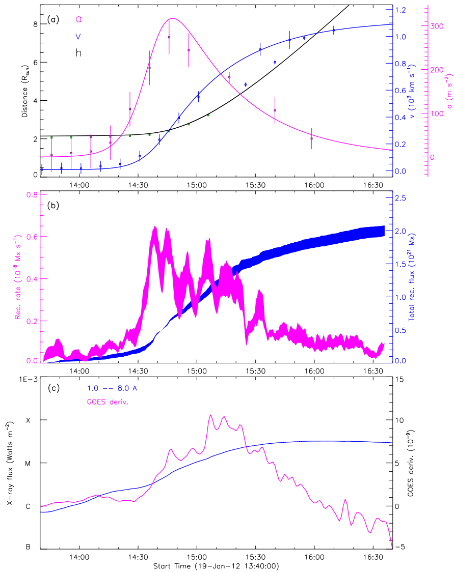
Figure 21: 20120119_13_STB195_rec_wavelnth.1600_GOES_used
