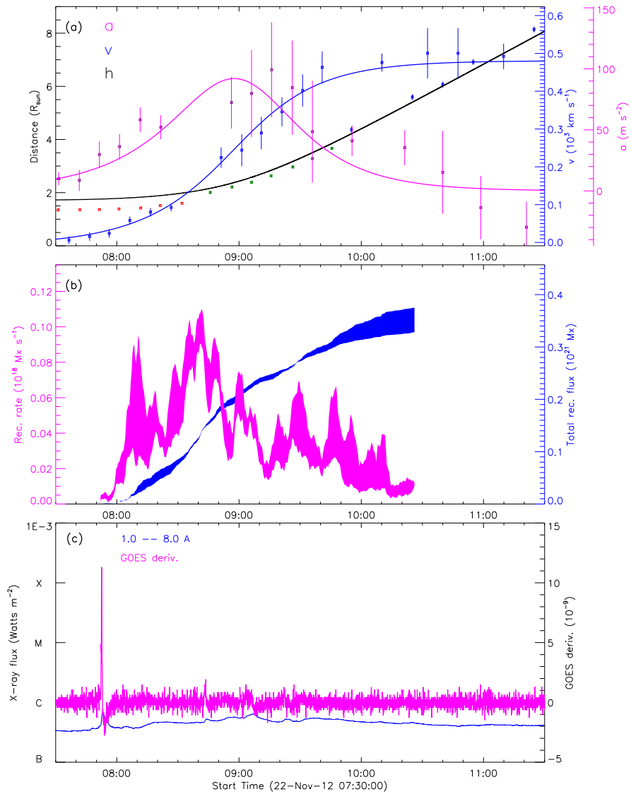
Figure 40: 20121122.08_STB195_rec_wavelnth_304_GOES_not_used
