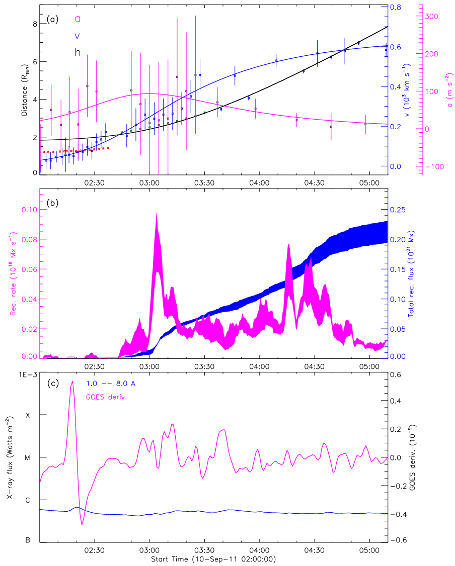
Figure 10: 20110910_STA171_rec_wavelnth_304_GOES_not_used
