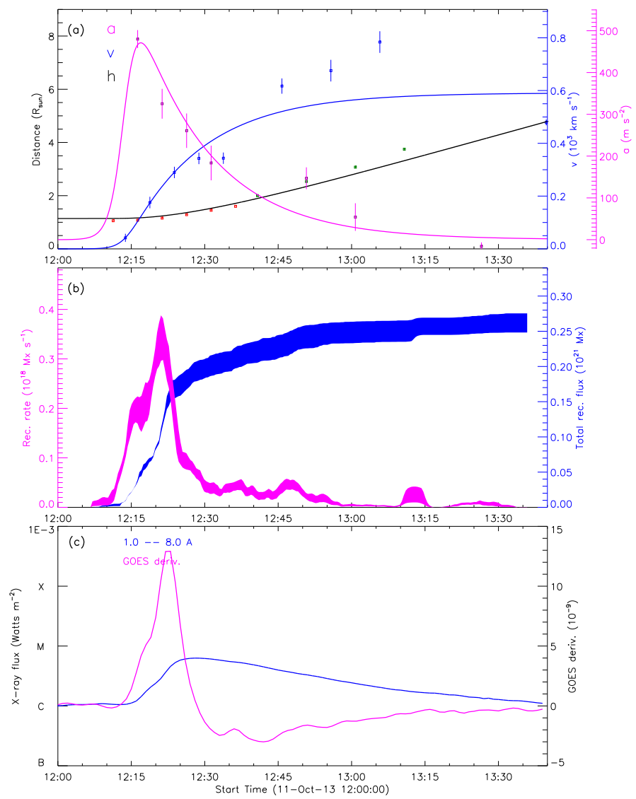
Figure 50: 20131011.12_STB195_rec_wavelnth.1600_GOES_used
