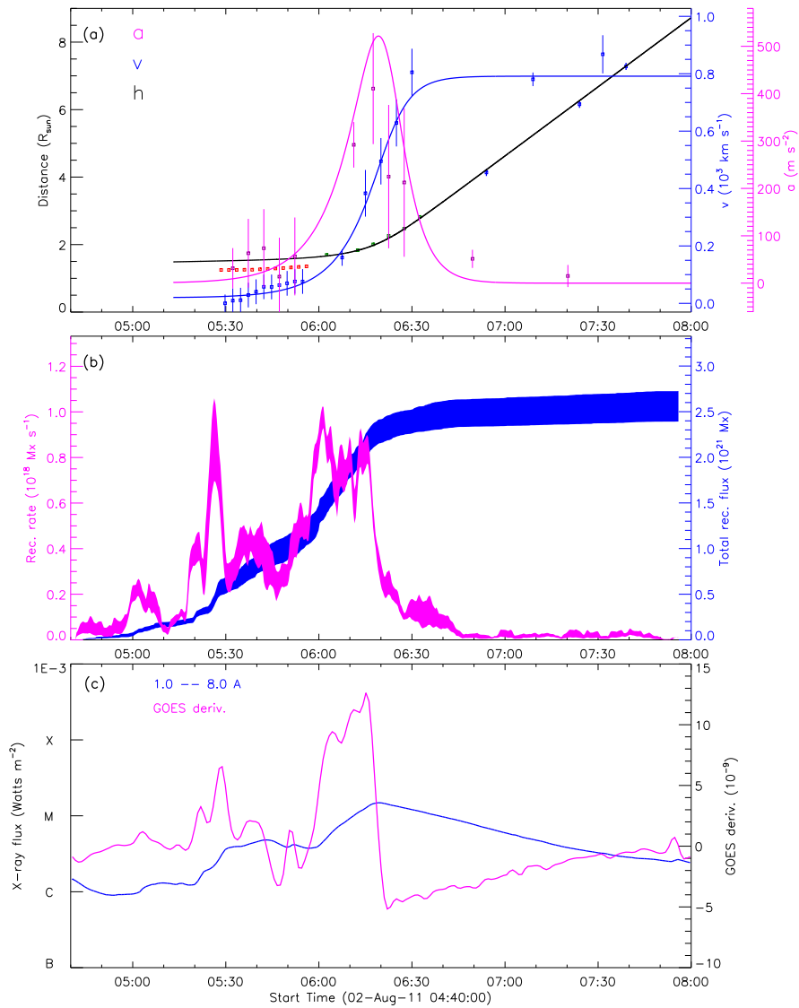
Figure 9: 20110802_STA171_rec_wavelnth_1600-GOES_used
