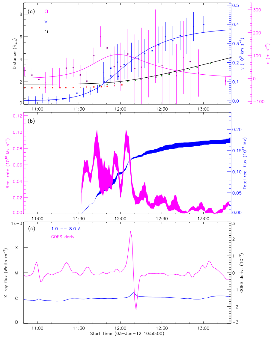
Figure 31: 20120603_12_STB195_rec_wavelnth_1600_GOES_not_used
