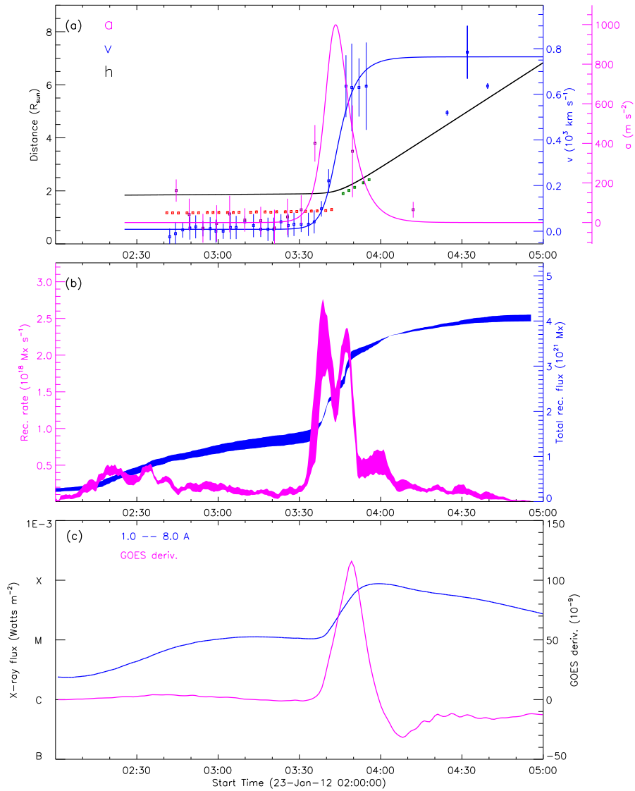
Figure 22: 20120123_STB171_rec_wavelnth.1600_GOES_used
