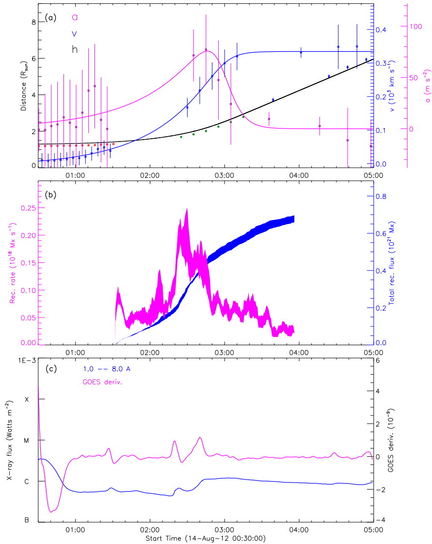
Figure 34: 20120814_STA195_rec_wavelnth_304_GOES_not_used
