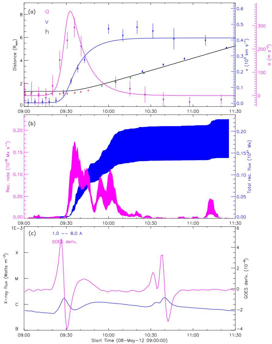
Figure 30: 20120508_STA195_rec_wavelnth_1600-GOES_not_used
