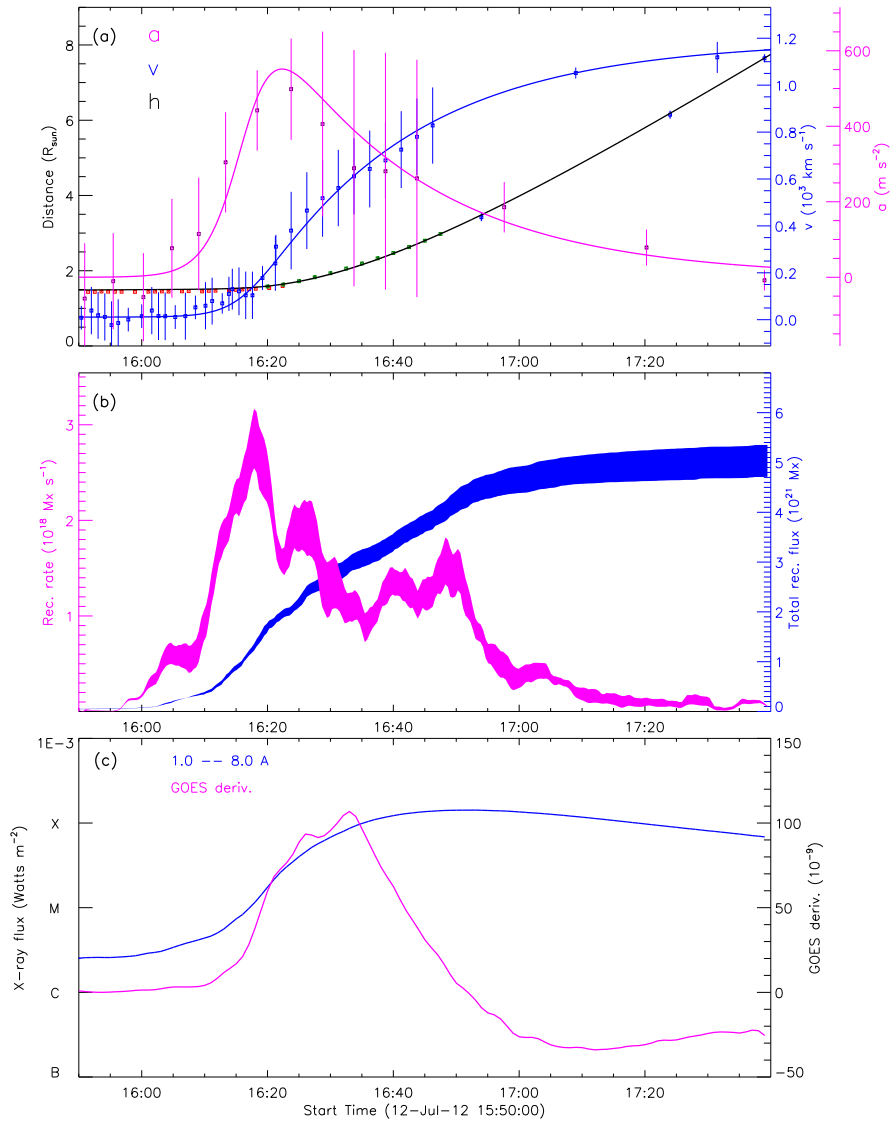
Figure 33: 20120712_STA171_rec_wavelnth_1600_GOES_used
