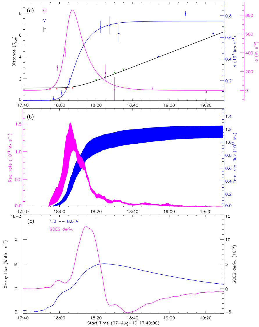
Figure 2: 20100807_STA171_rec_wavelnth_1600-GOES_used
