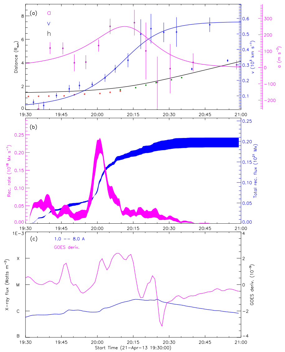
Figure 47: 20130421_20_STA195_rec_wavelnth.1600_GOES_used
