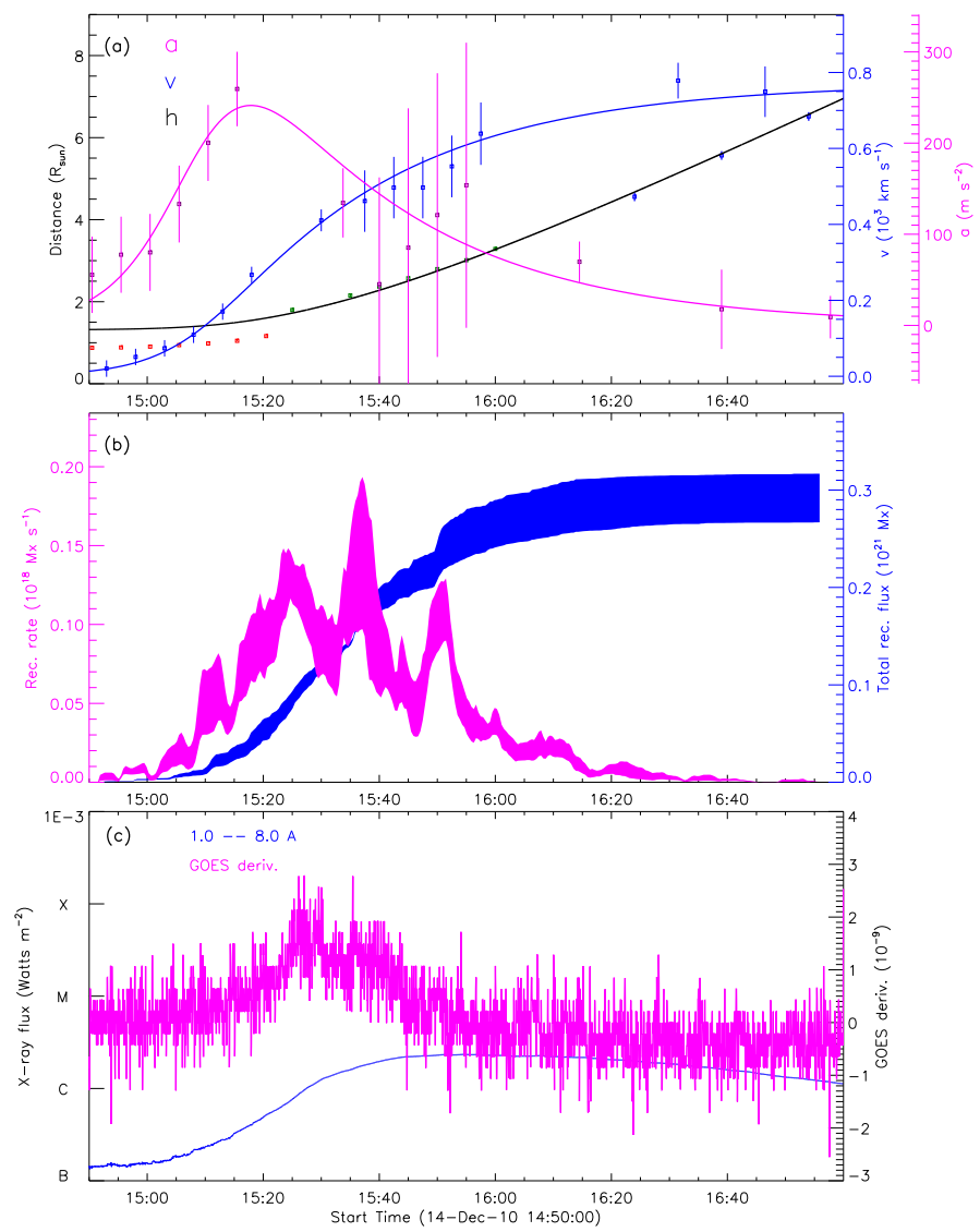
Figure 5: 20101214_STA195_rec_wavelnth_1600-GOES_used
