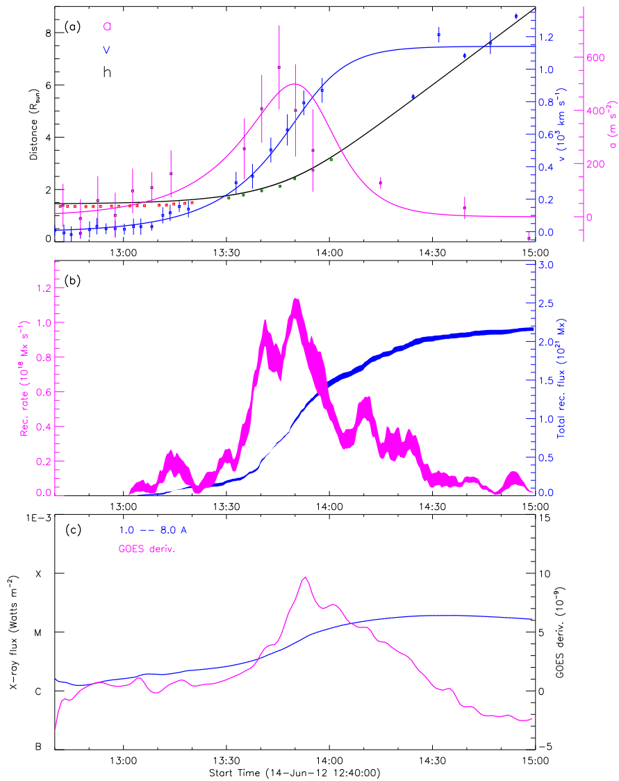
Figure 32: 20120614_STB171_rec_wavelnth.1600_GOES_used
