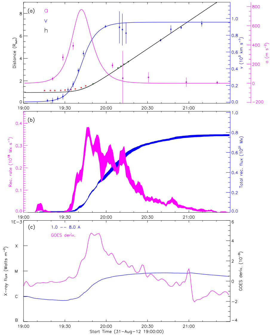
Figure 36: 20120831_STB171_rec_wavelnth.1600_GOES_used
