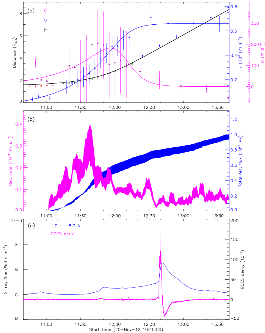
Figure 57: 20121120_11_STA195_rec_wavelnth_304_GOES_not_used
