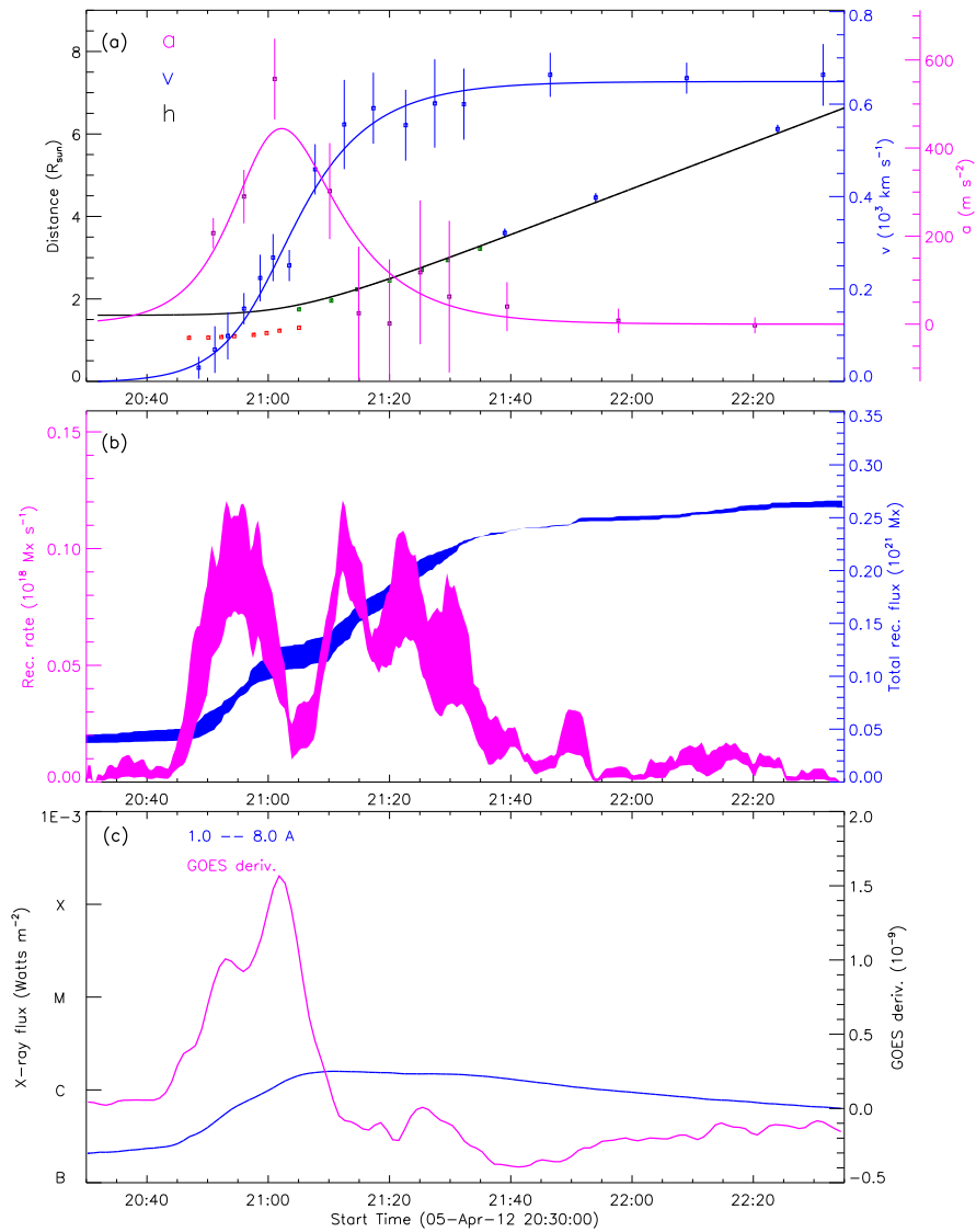
Figure 27: 20120405_STA171_rec_wavelnth_1600_GOES_used
