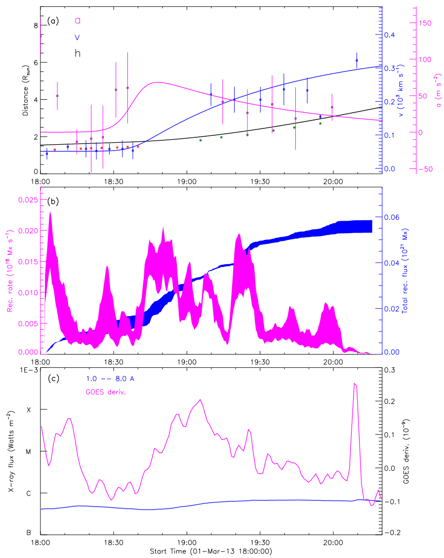
Figure 44: 20130301.17_STA195.rec.wavelnth.no_GOES_not_used
