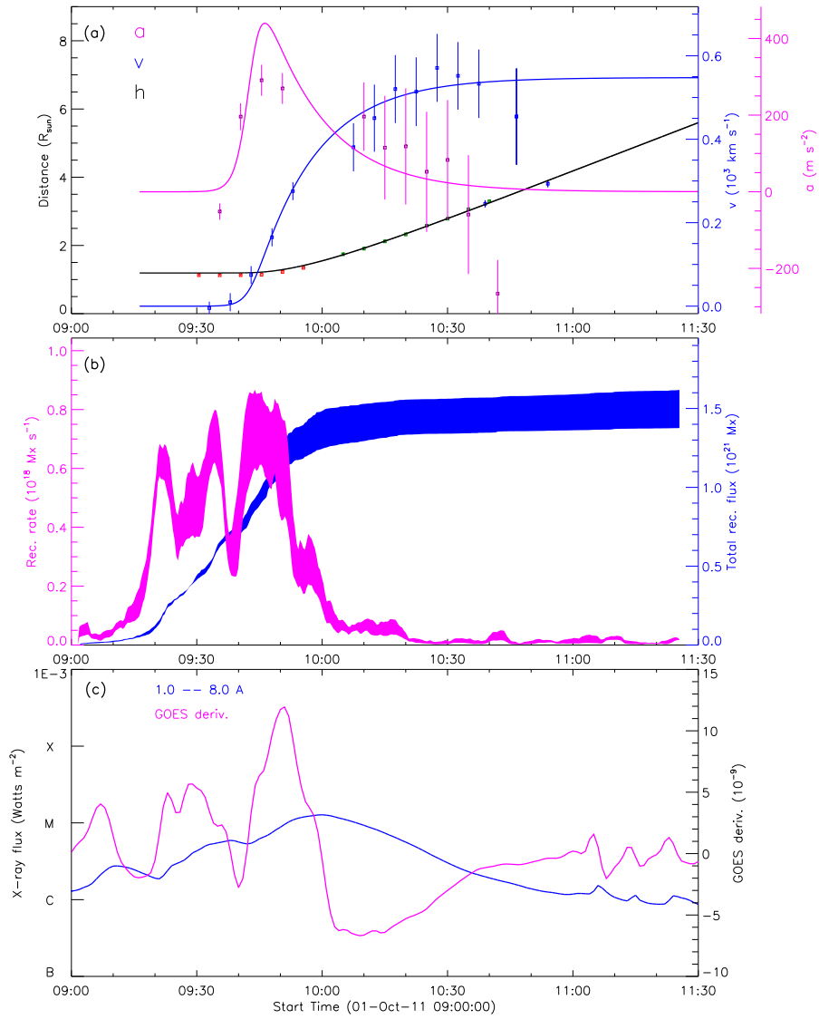
Figure 12: 20111001_STA195_rec_wavelnth_1600_GOES_used
