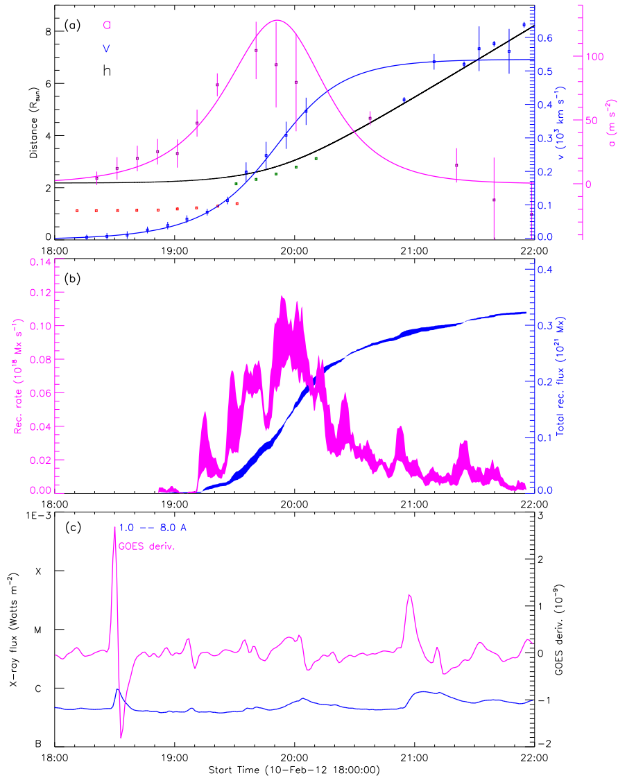
Figure 23: 20120210.19_STB195_rec_wavelnth_no_GOES_not_used
