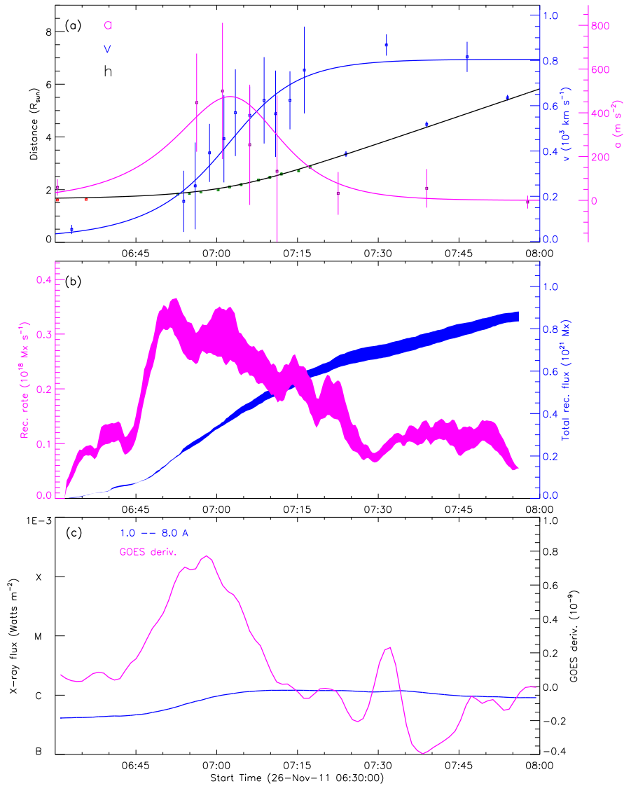
Figure 16: 20111126_STA195_rec_wavelnth_304_GOES_used
