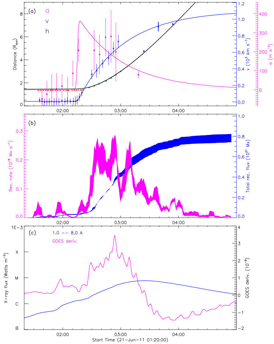
Figure 7: 20110621_STA171_rec_wavelnth_1600-GOES_used
