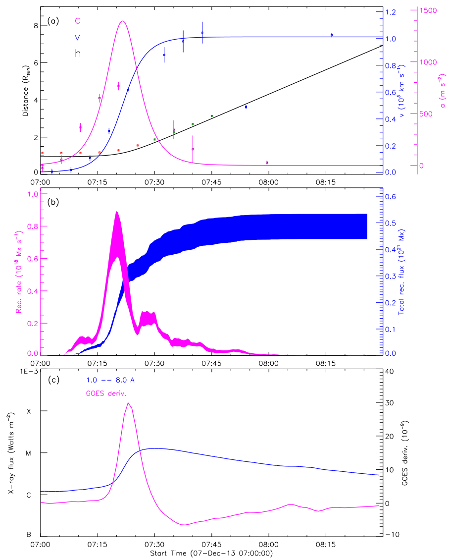
Figure 52: 20131207_07_STA195_rec_wavelnth.1600_GOES_used
