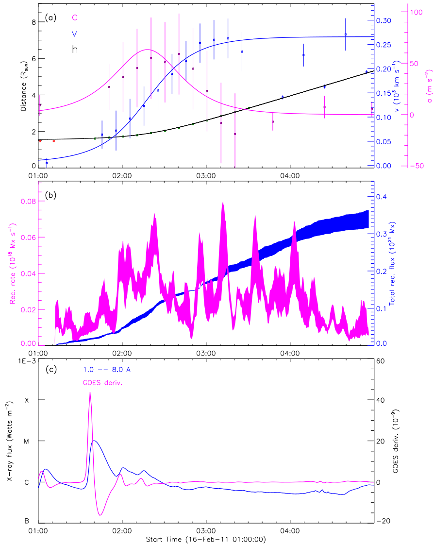
Figure 6: 20110216_01.STB195_rec_wavelnth_304_GOES_other_region
