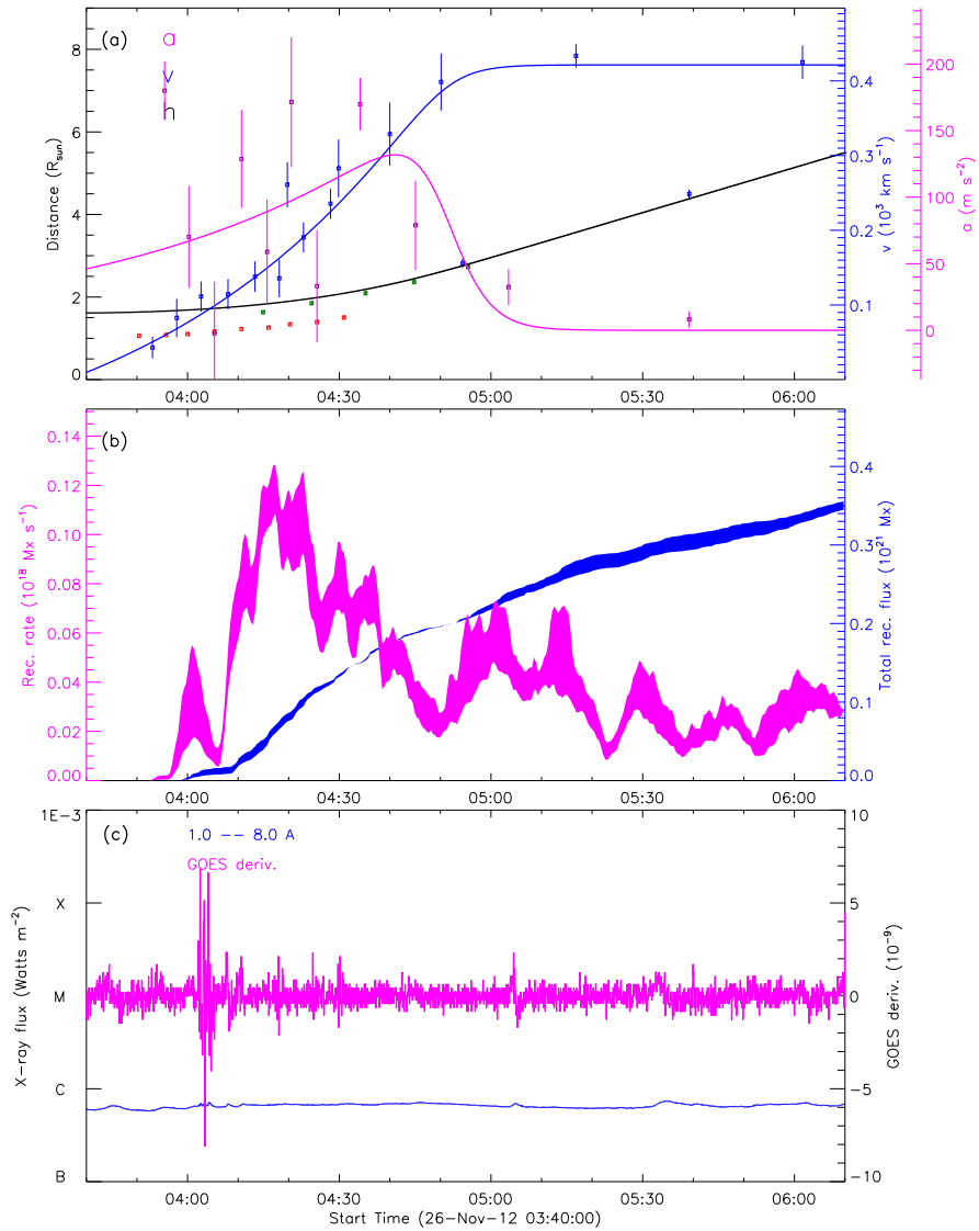
Figure 41: 20121126_04_STA195_rec_wavelnth_304_GOES_not_used
