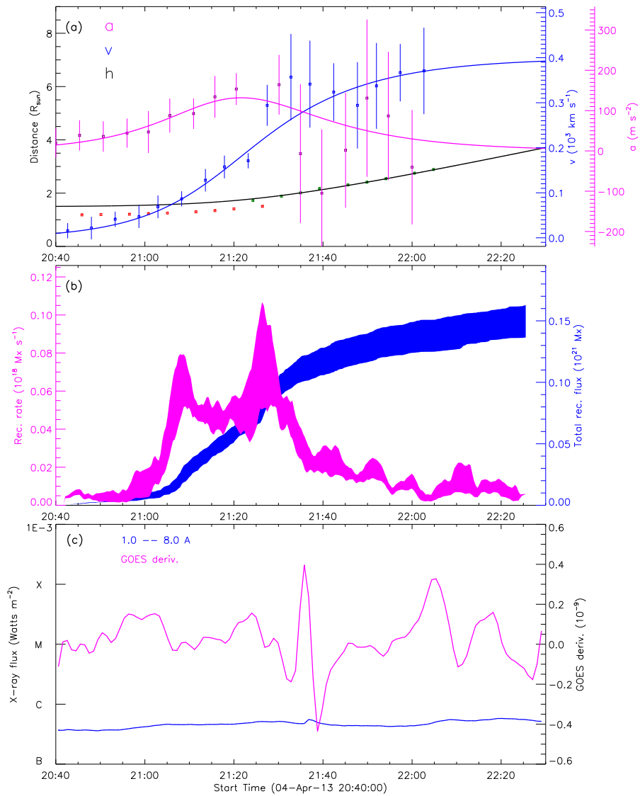
Figure 46: 20130404_STA195_rec_wavelnth_no_GOES_not_used
