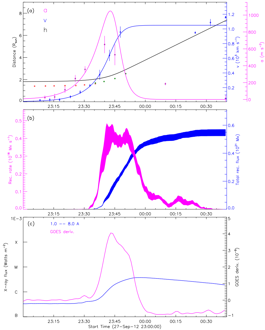
Figure 37: 20120927_23_STA195_rec_wavelnth.1600_GOES_used
