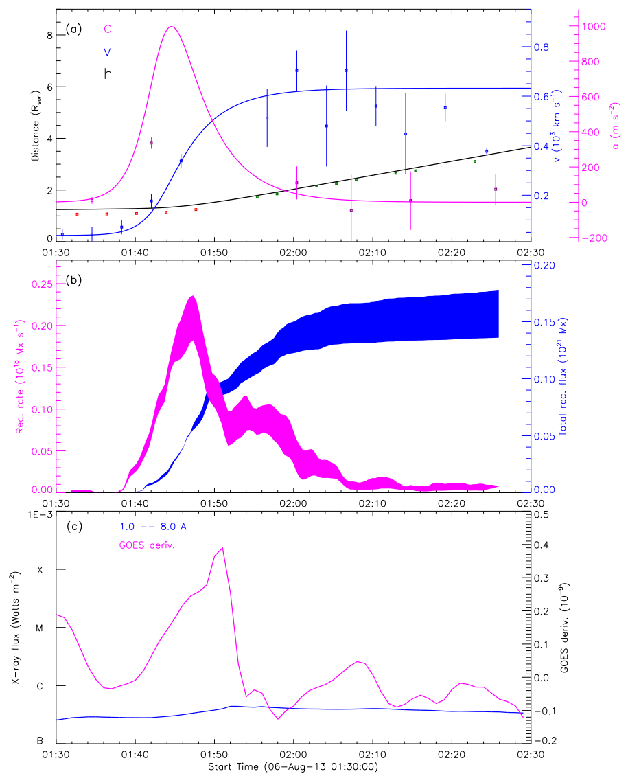
Figure 48: 20130806_STB171_rec_wavelnth_304_GOES_used
