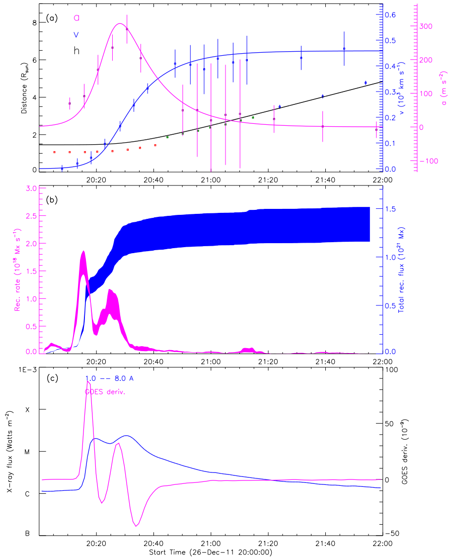
Figure 19: 20111226_STA195_rec_wavelnth_1600_GOES_used
