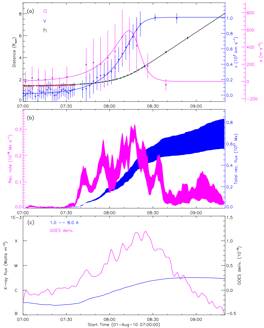
Figure 1: 20100801_STA171_rec_wavelnth_1600-GOES_used
