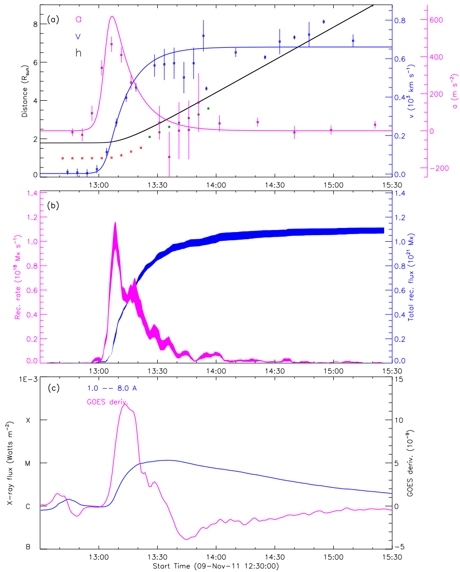
Figure 14: 20111109_12_STB195_rec_wavelnth.1600_GOES_used
