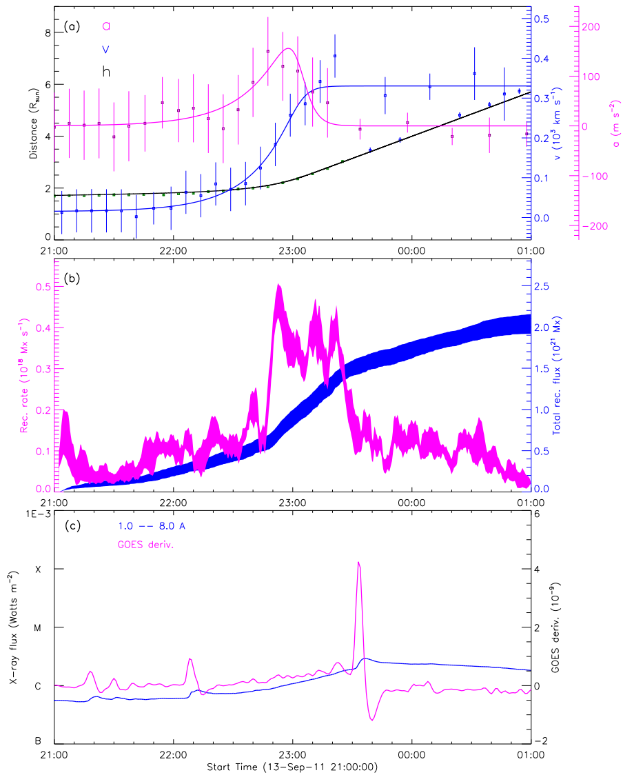
Figure 11: 20110913_STA171_rec_wavelnth_304_GOES_not_used
