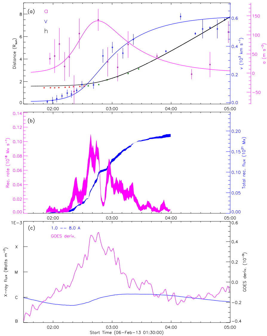
Figure 42: 20130206_00_STB195_rec_wavelnth.1600_GOES_used
