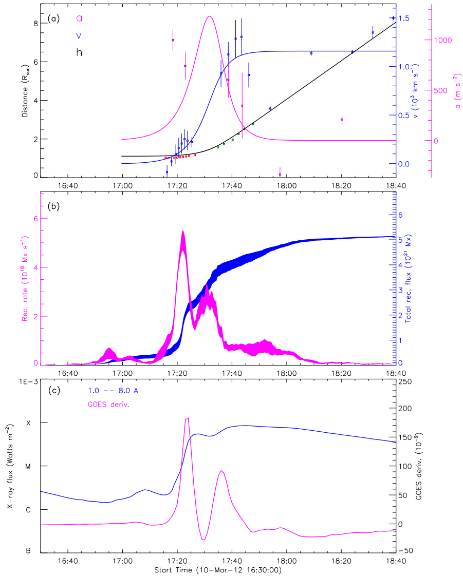
Figure 26: 20120310.16_STA171_rec_wavelnth.1600_GOES_used
