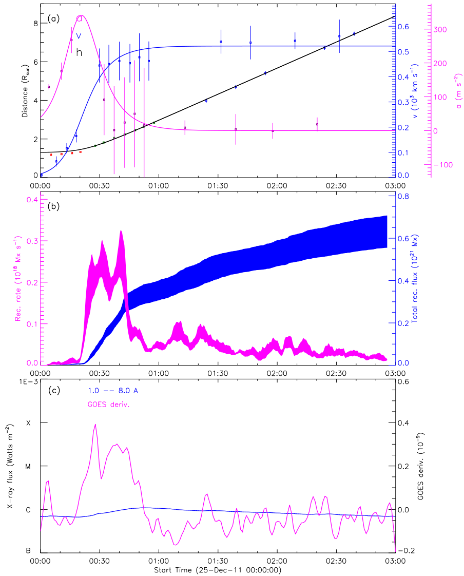
Figure 17: 20111225_00_STA195_rec_wavelnth_304_GOES_used
