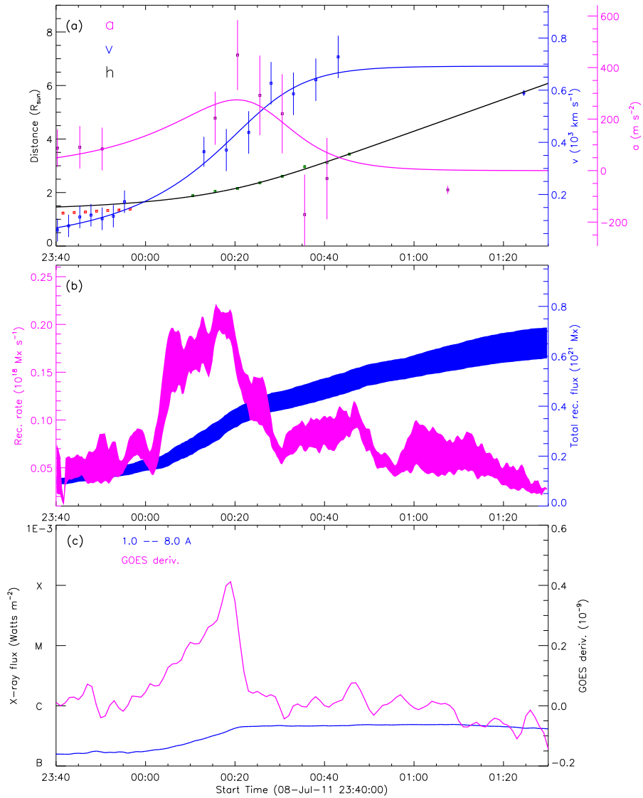
Figure 8: 20110708_STB171_rec_wavelnth_304_GOES_used
