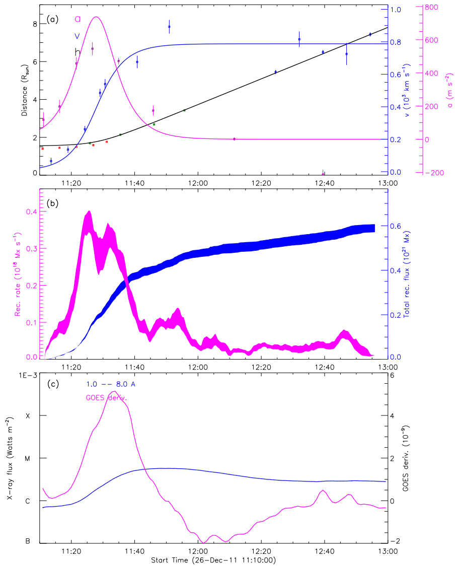
Figure 18: 20111226_11_STB195_rec_wavelnth.1600_GOES_used
