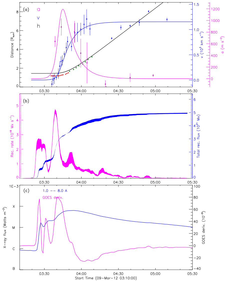
Figure 25: 20120309_STB171_rec_wavelnth.1600_GOES_used
