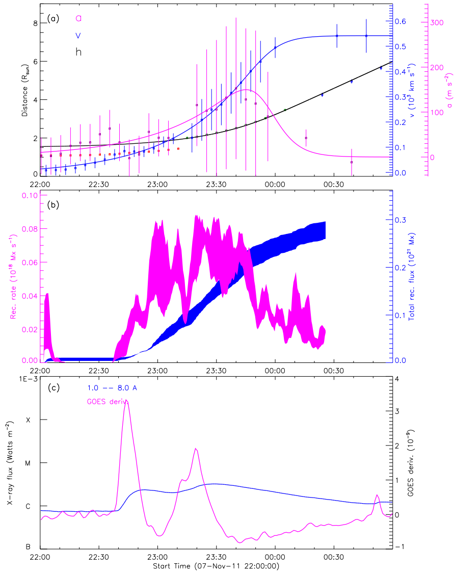
Figure 13: 20111107_STA195_rec_wavelnth_304_GOES_other_region
