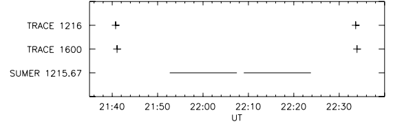
Fig. 1. Epochs and durations of the images analyzed in the present study. The integration times of the TRACE observations are too short to be shown in the plot, and those observations are denoted with crosses.
