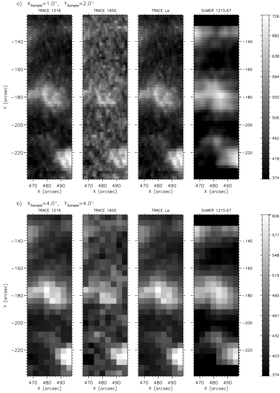
Fig. 2. TRACE and SUMER images with a sampling size of a) 1'' \times 2'' and b) 4'' \times 4'' . TRACE L\alpha image is obtained by using Eq. (1) with the best-fit B value of a) -0.036 and b) -0.120 . The bars indicate the intensities of the grayscale in units of count per second for TRACE 1216 images. The grayscale for other images are appropriately scaled for ease of comparison.
