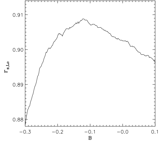
Fig. 3. r_{s,L\alpha} values as a function of B for a sampling size of 4'' \times 4'' and X_{\text{shift}} = 2.0'' and Y_{\text{shift}} = -2.6'' . These X_{\text{shift}} and Y_{\text{shift}} values maximize r_{s,L\alpha} as described in the text.
