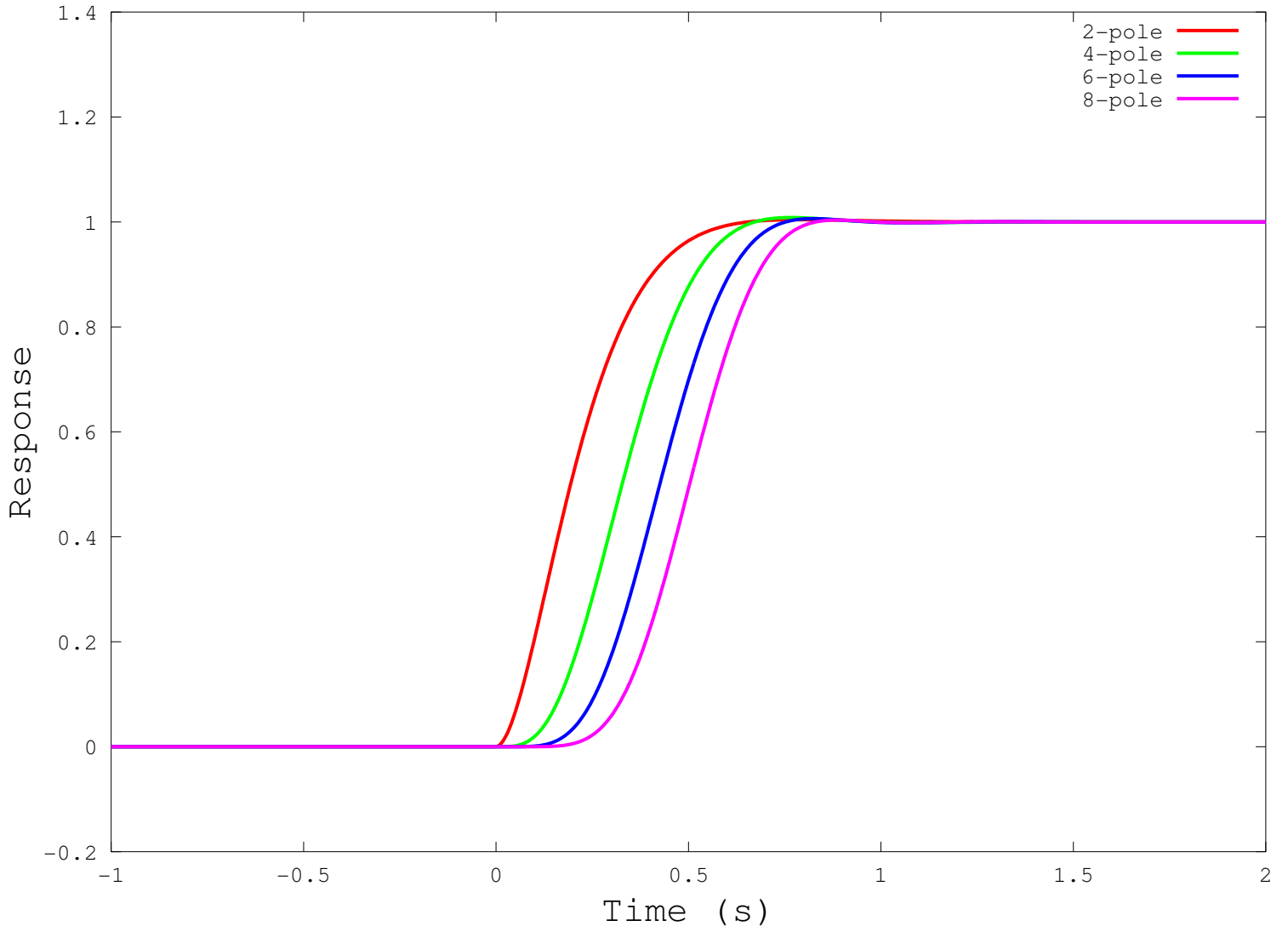
Step response of Bessel filters
