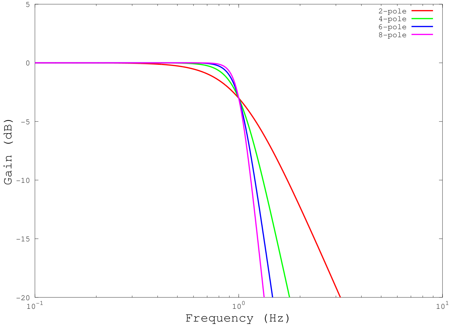
Gain of Butterworth filters
