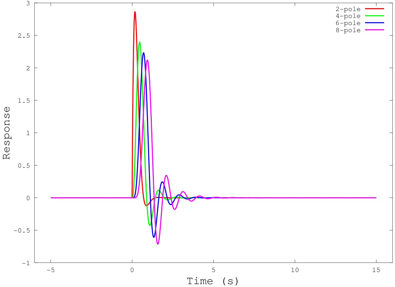
Impulse response of Butterworth filters
