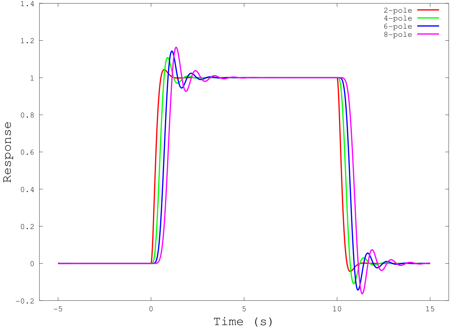
Step response of Butterworth filters
