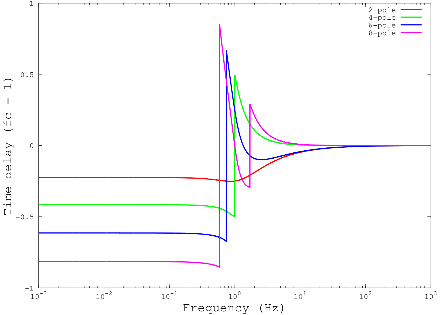
Time delay of Butterworth filters
