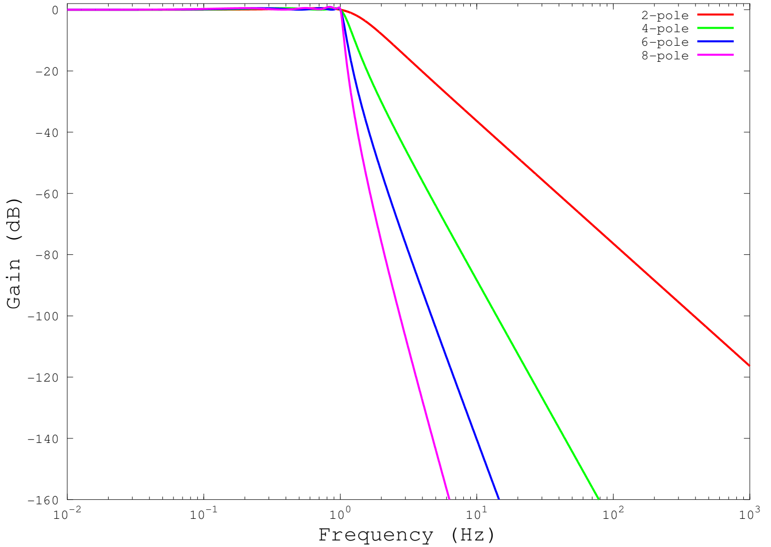
Gain of Chebyshev (0.5 dB) filters
