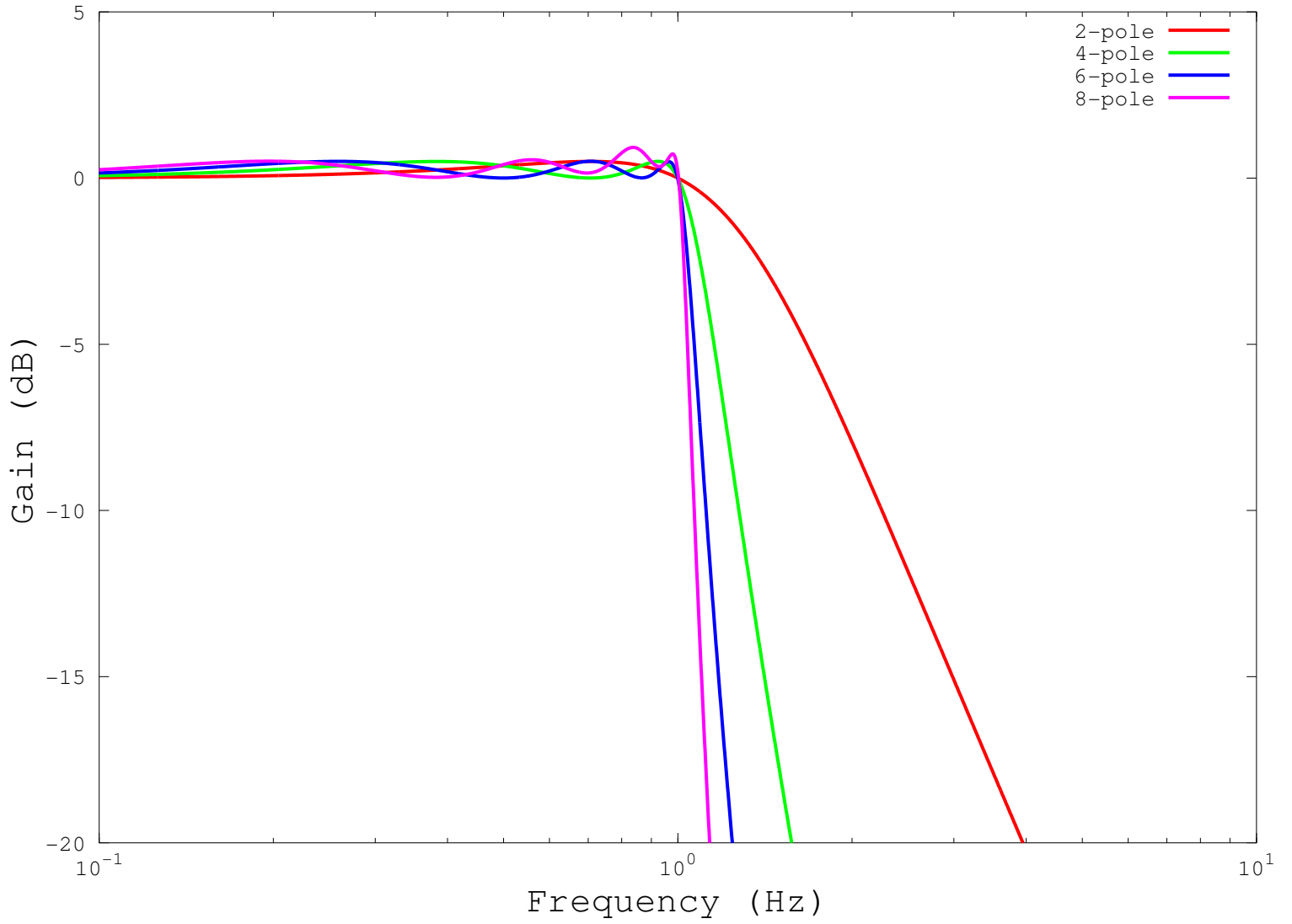
Gain of Chebyshev (0.5 dB) filters
