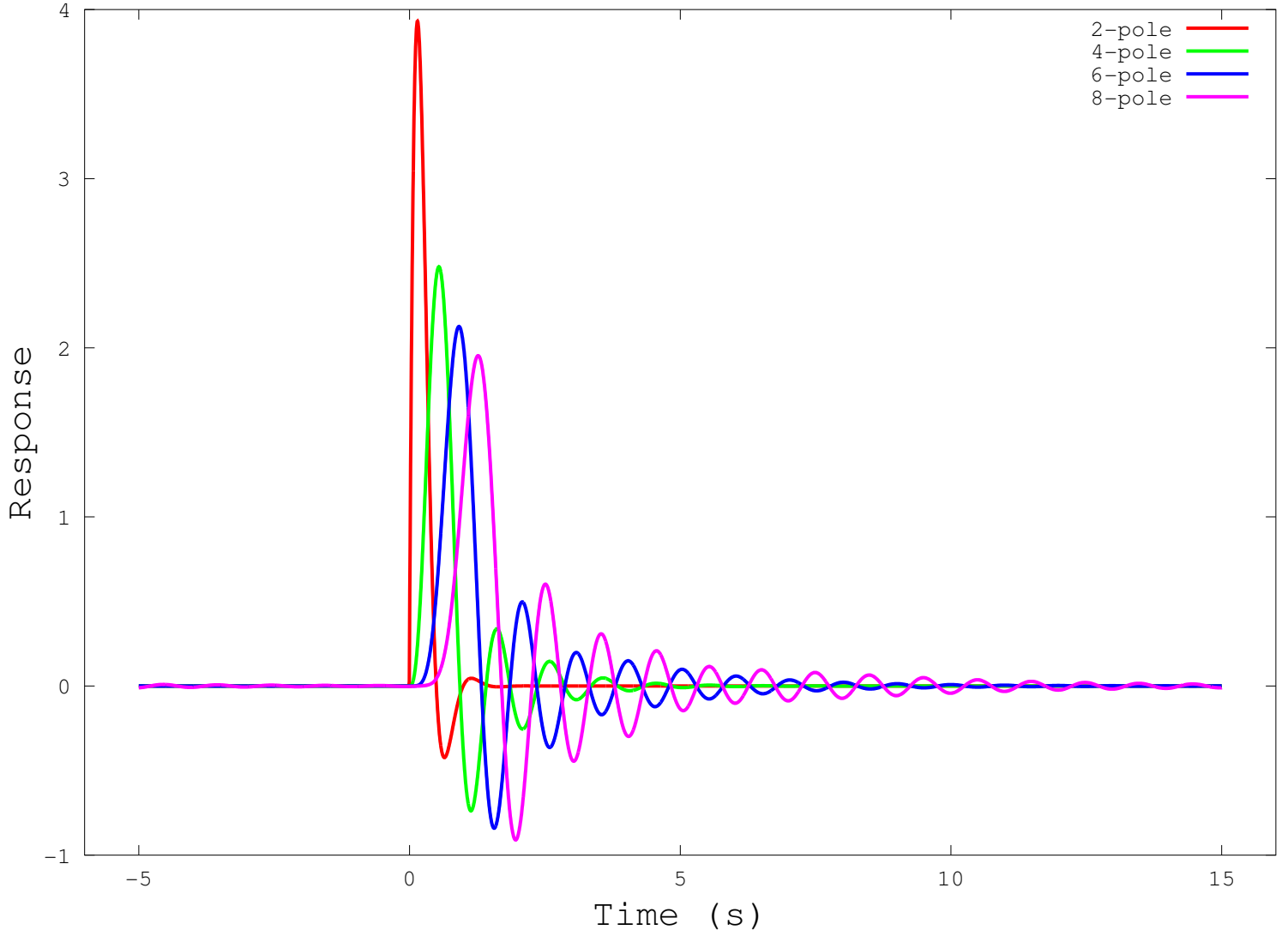
Impulse response of Chebyshev (0.5 dB) filters
