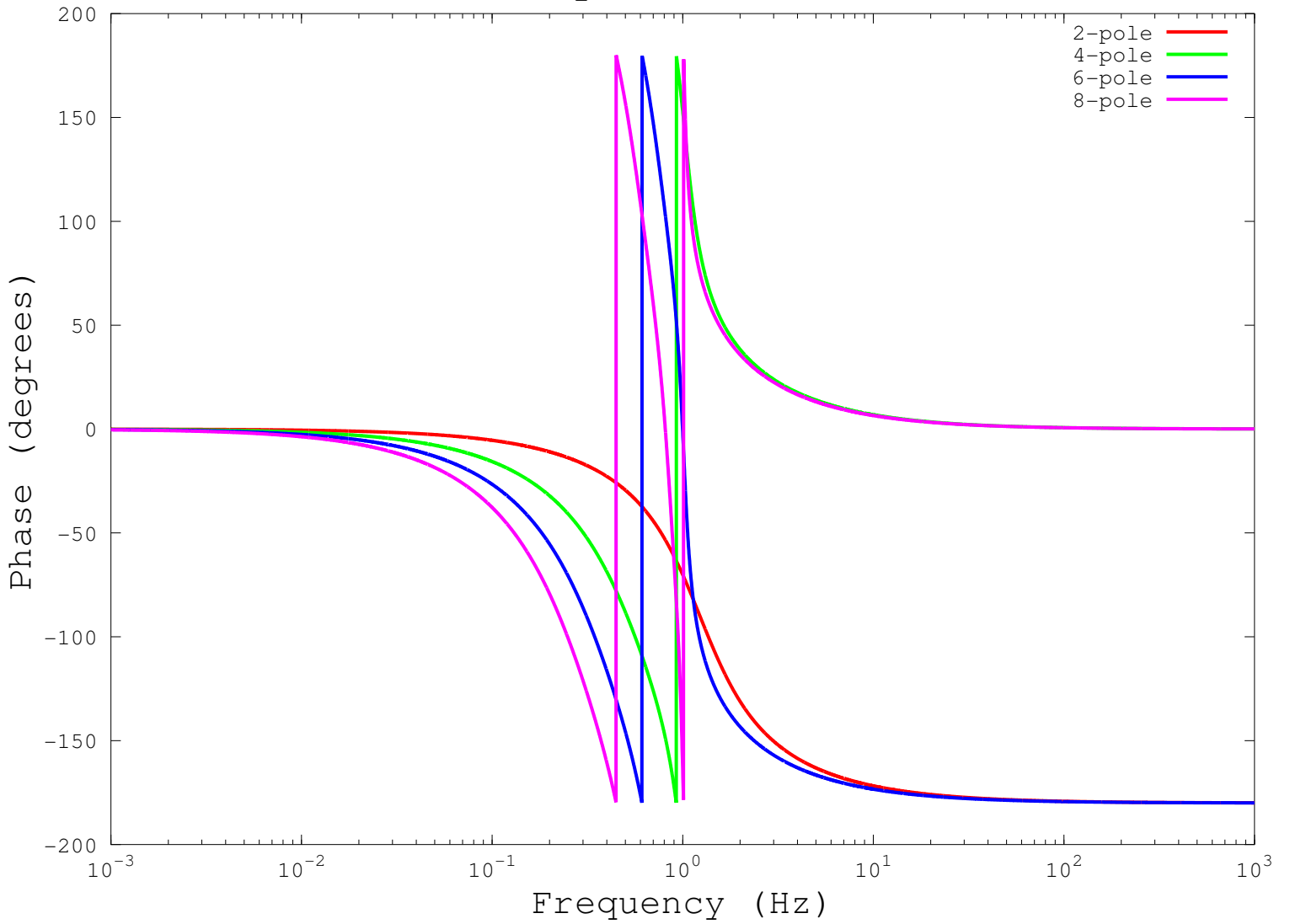
Phase of Chebyshev (0.5 dB) filters
