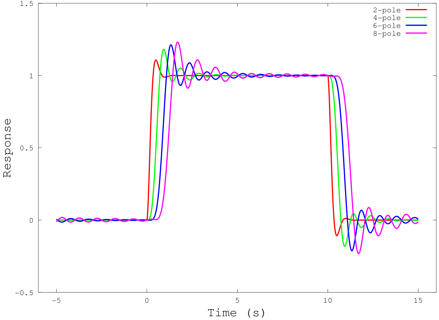
Step response of Chebyshev (0.5 dB) filters
