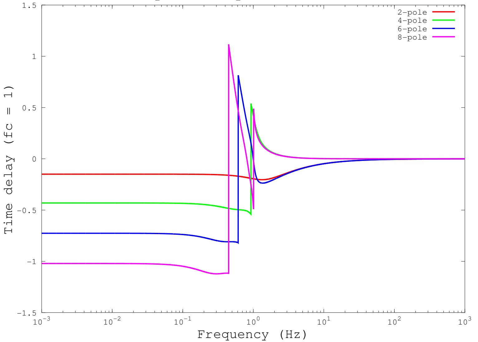
Time delay of Chebyshev (0.5 dB) filters
