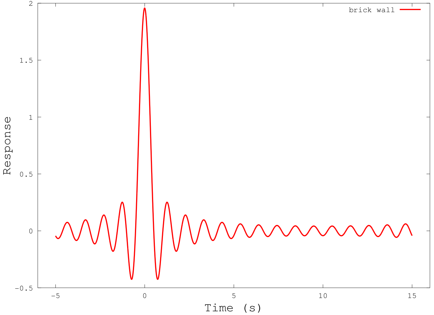
Impulse response of brick wall filter
