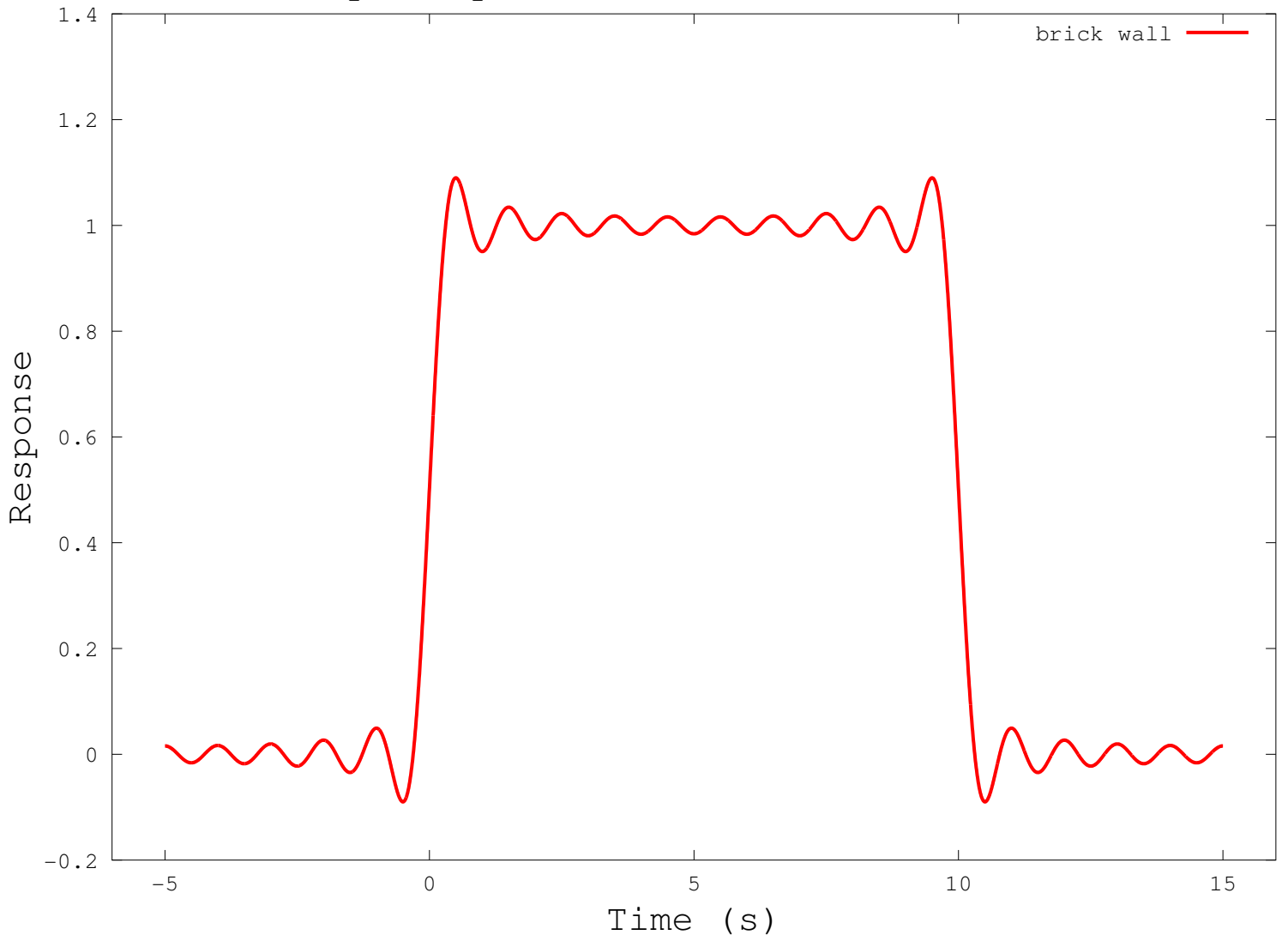
Step response of brick wall filter
