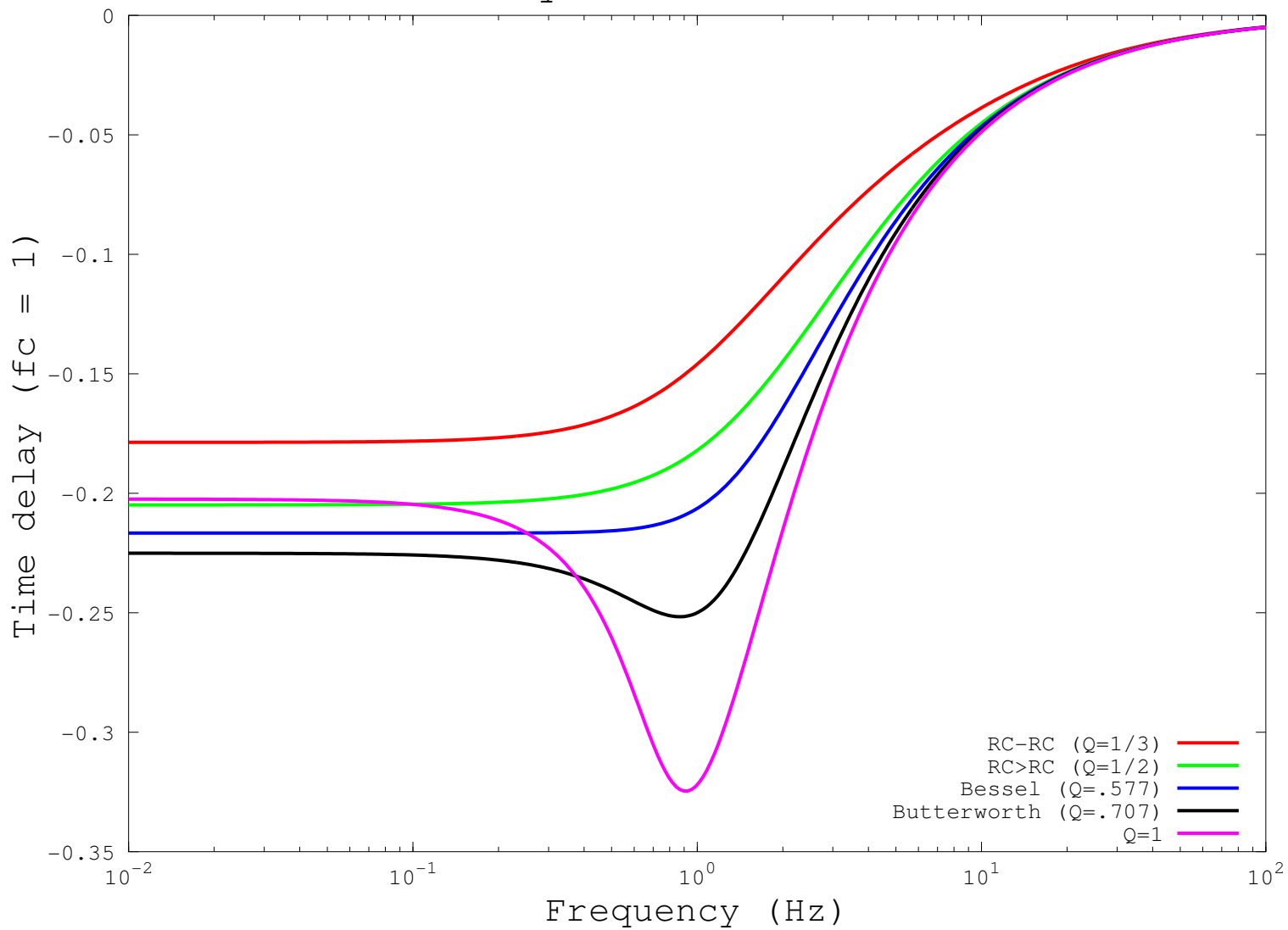
Time delay of 2nd order filters
