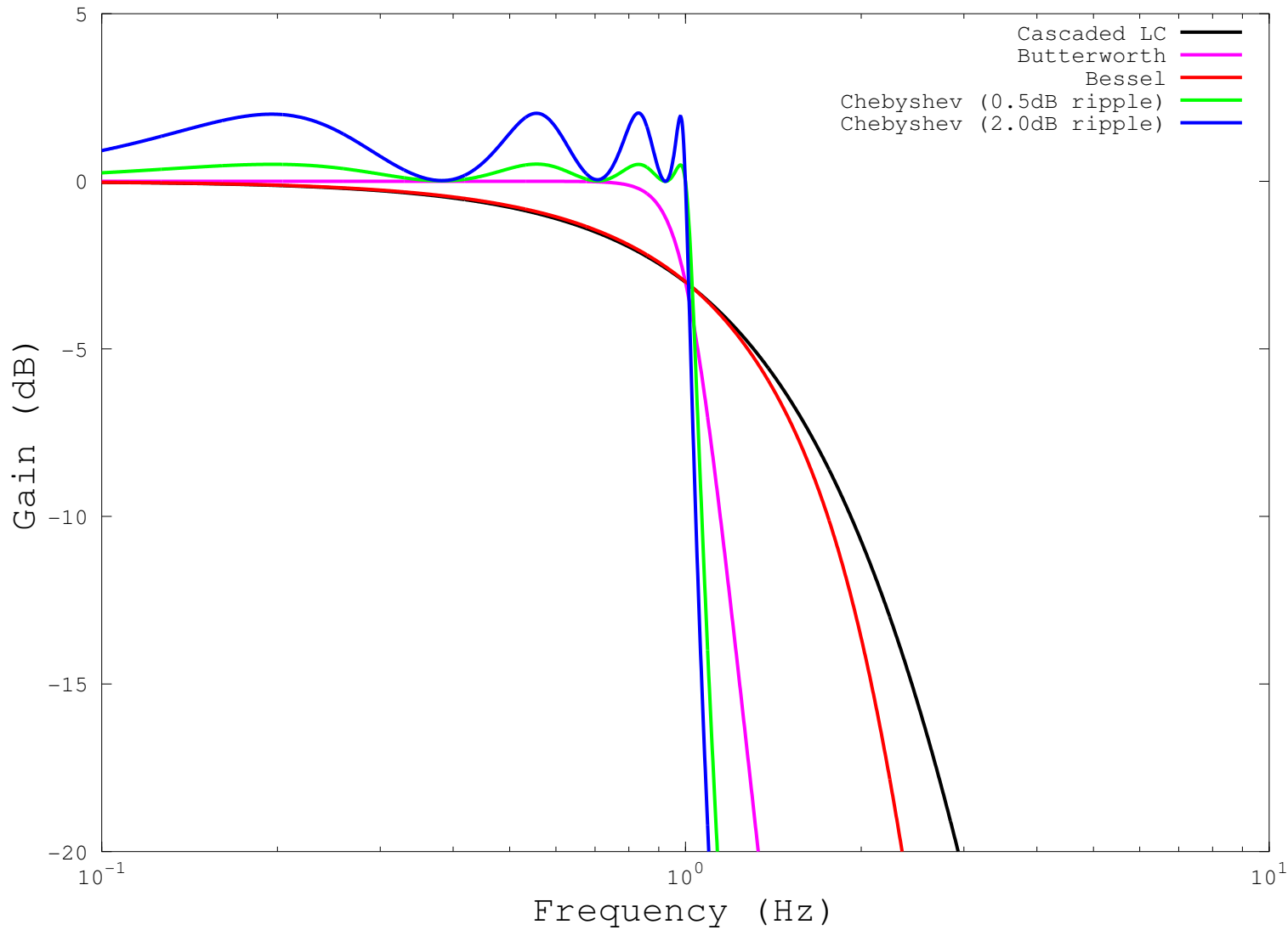
Gain of 8th-order filters
