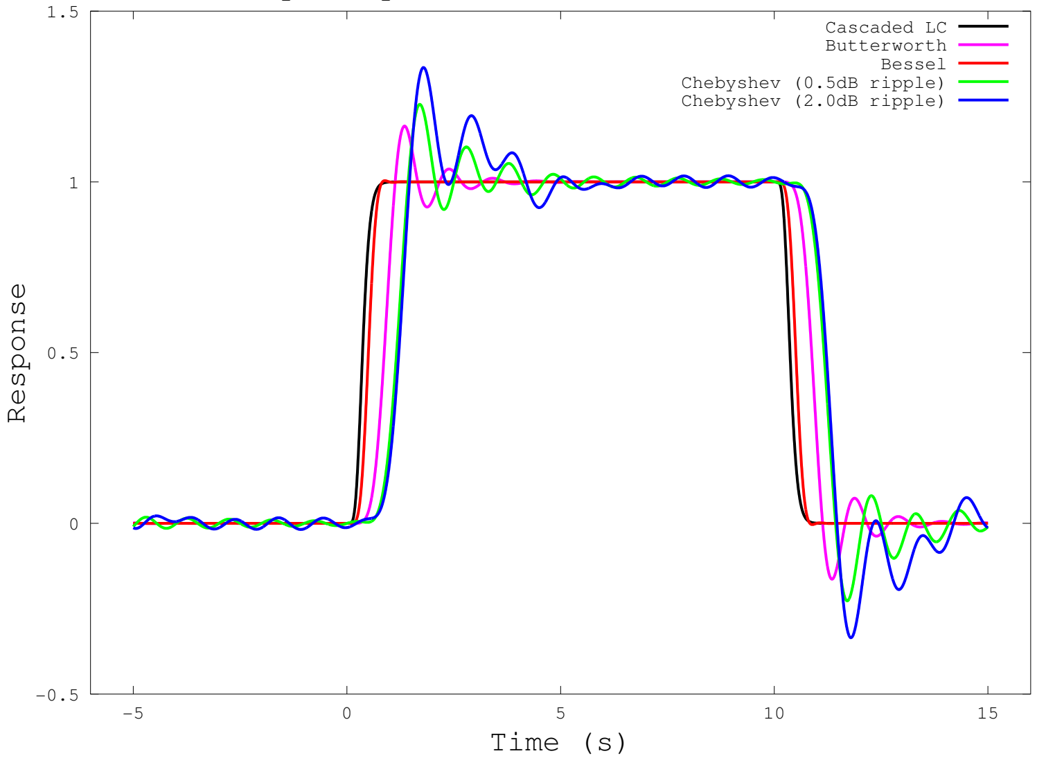
Step response of 8th order filters
