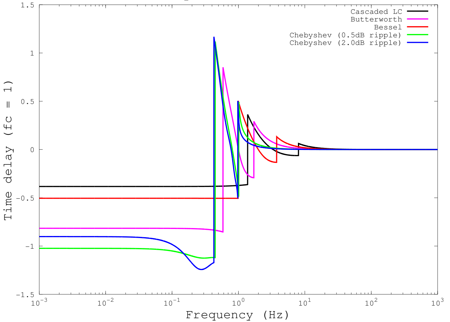
Time delay of 8th order filters
