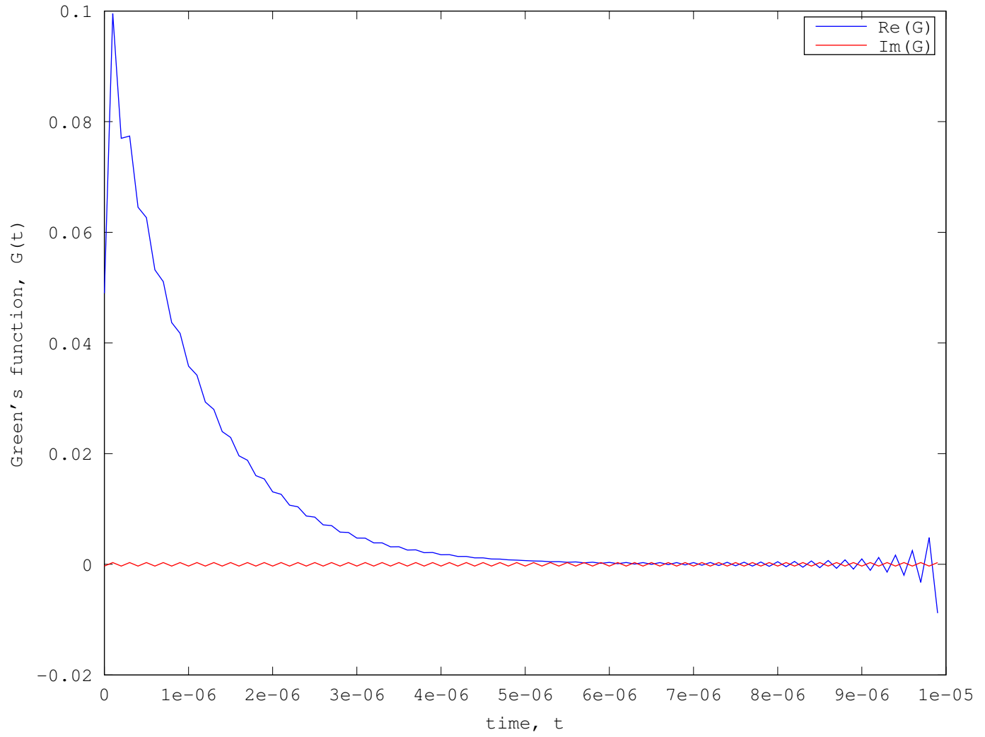
Green's Function for Lowpass Filter, RC = 1 \mu s
