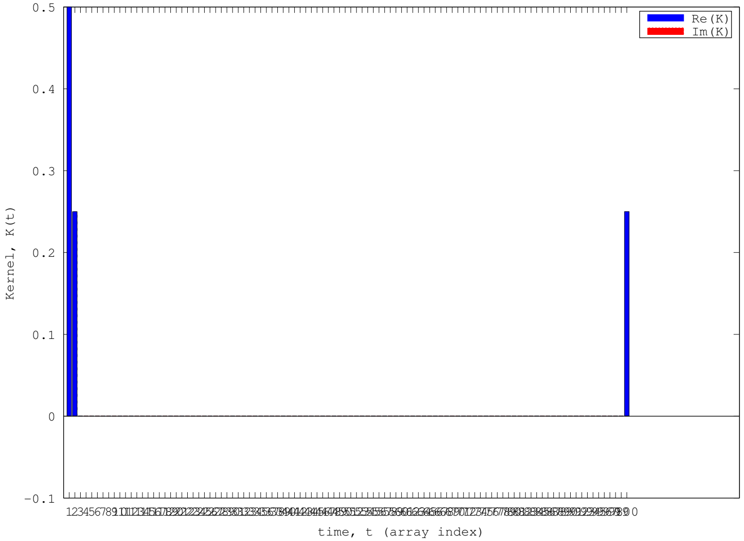
Convolution kernel of the anti-aliasing filter
