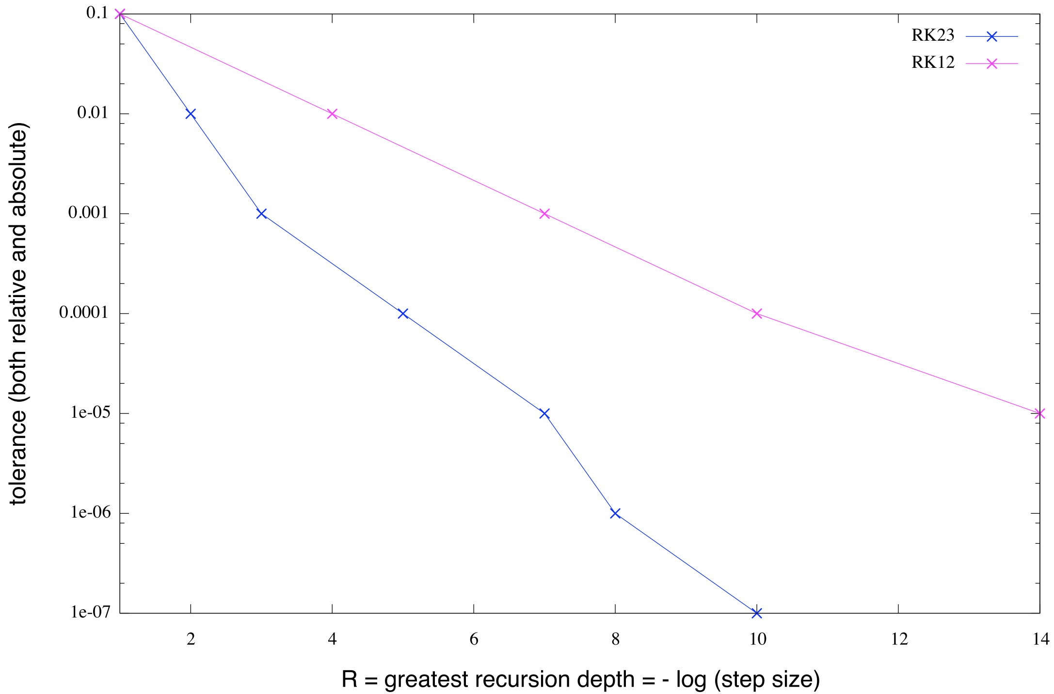
adaptive_test1.m: performance of adaptive_stepper
