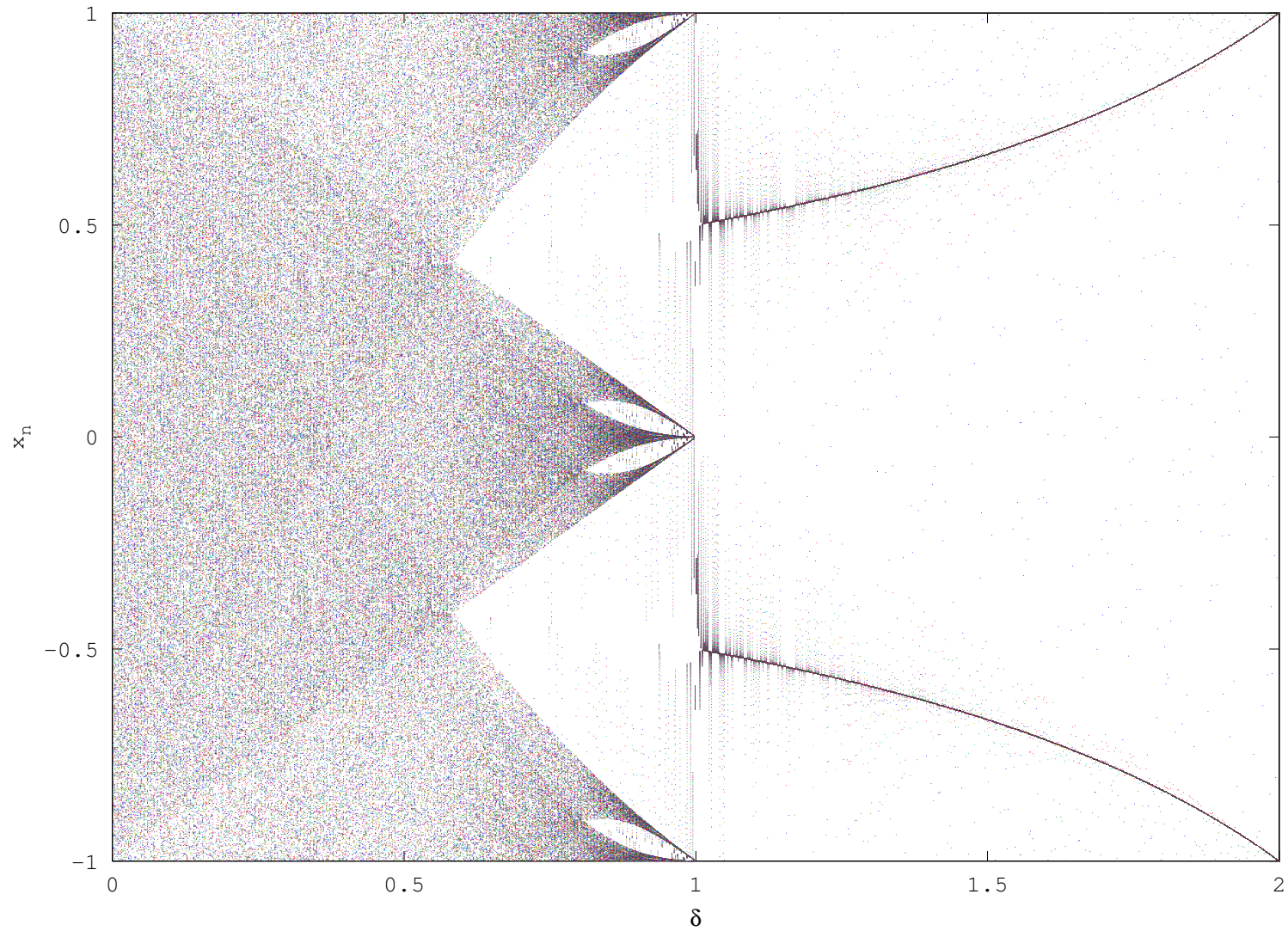
Card Shuffling: Bifurcation Diagram
