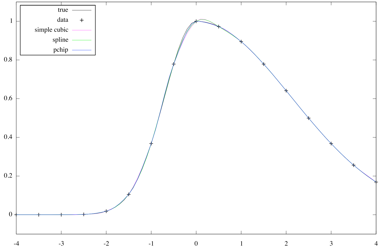
Piecewise Gaussians, factor of 3 change in 2nd deriv at origin.
