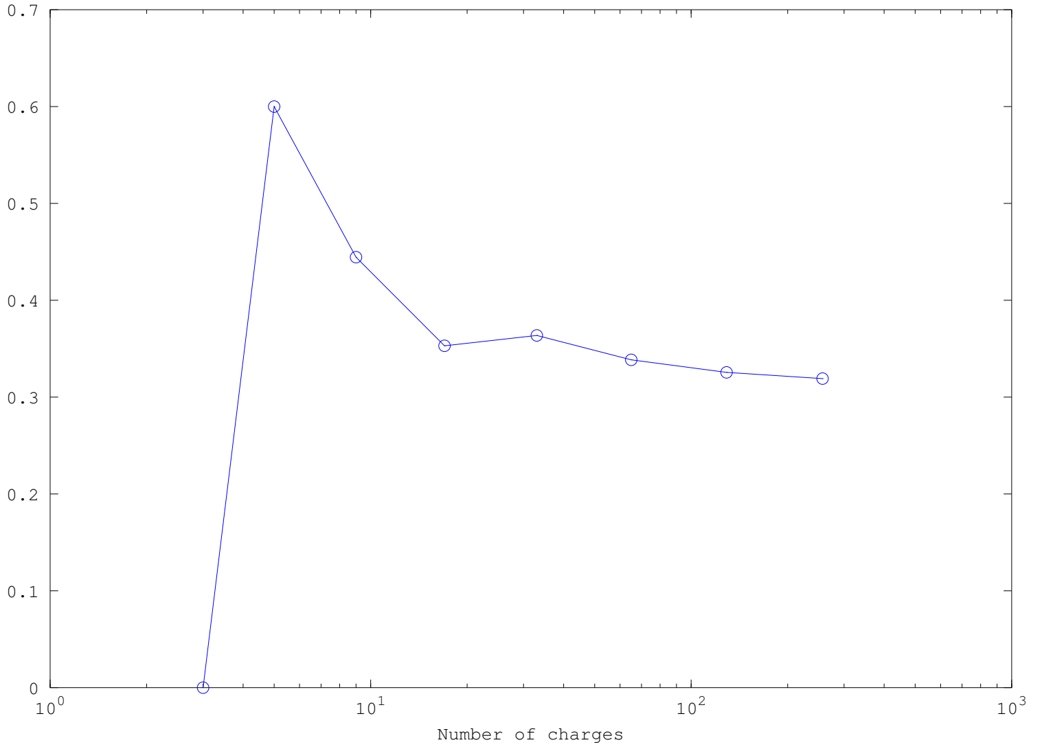
Fraction of charge in density-enhanced regions ( \lambda > 1 )
