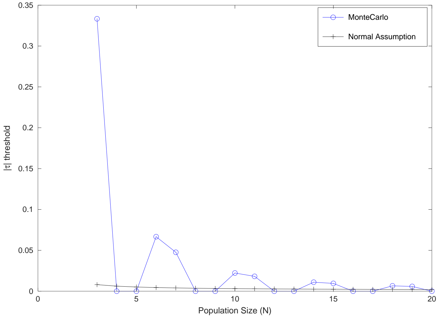
Kendall \tau , 1.00% Significance, 10000 Trials
