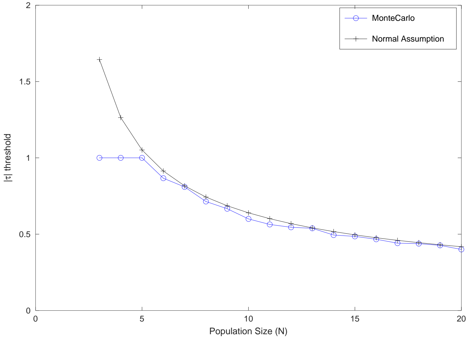
Kendall \tau , 99.00% Significance, 10000 Trials
