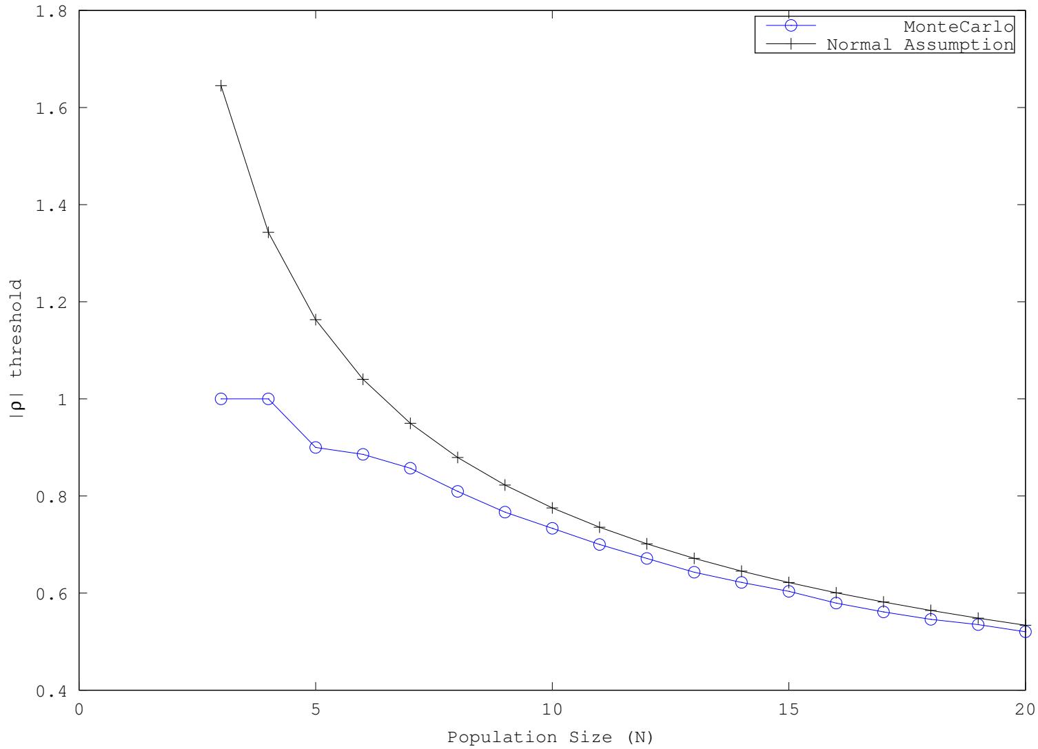
Spearman \rho , 98.00% Significance, 100000 Trials
