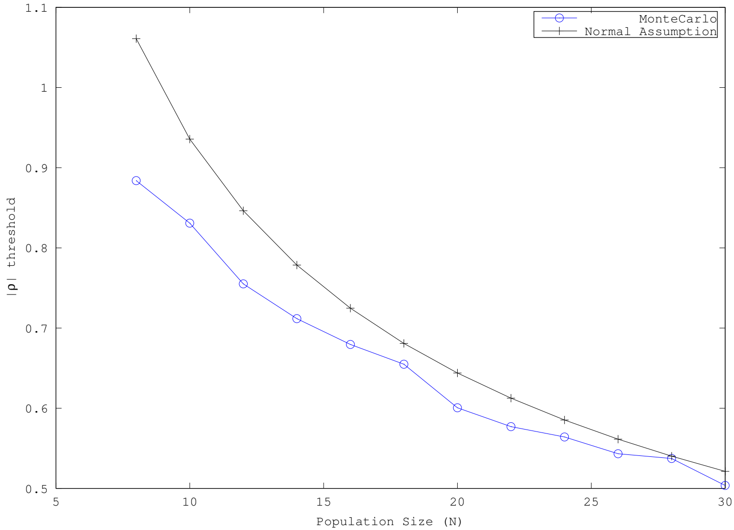
8-channel data: Spearman \rho , 99.50% Significance, 10000 Trials
