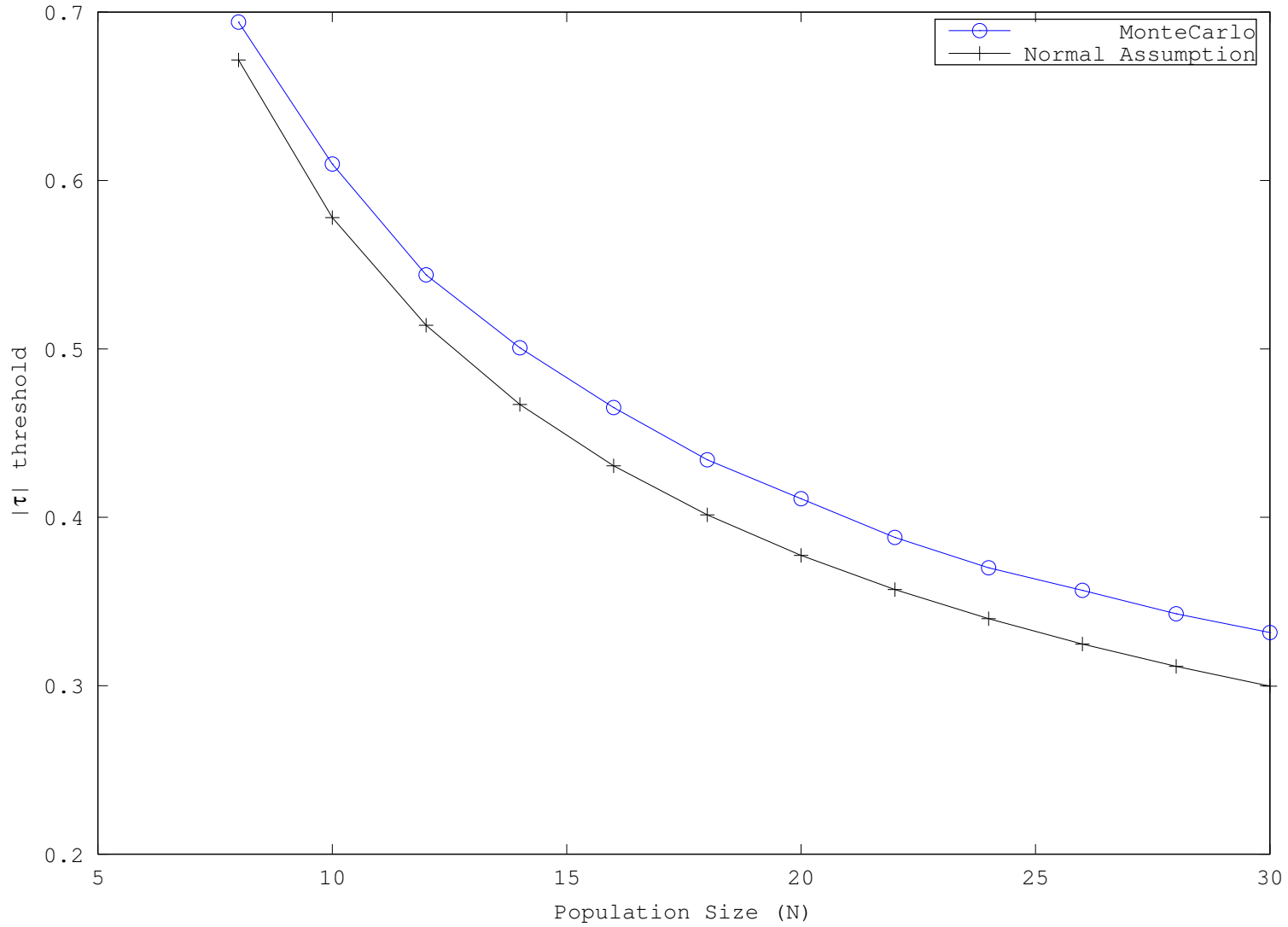
8-channel data: Kendall \tau , 98.00% Significance, 100000 Trials
