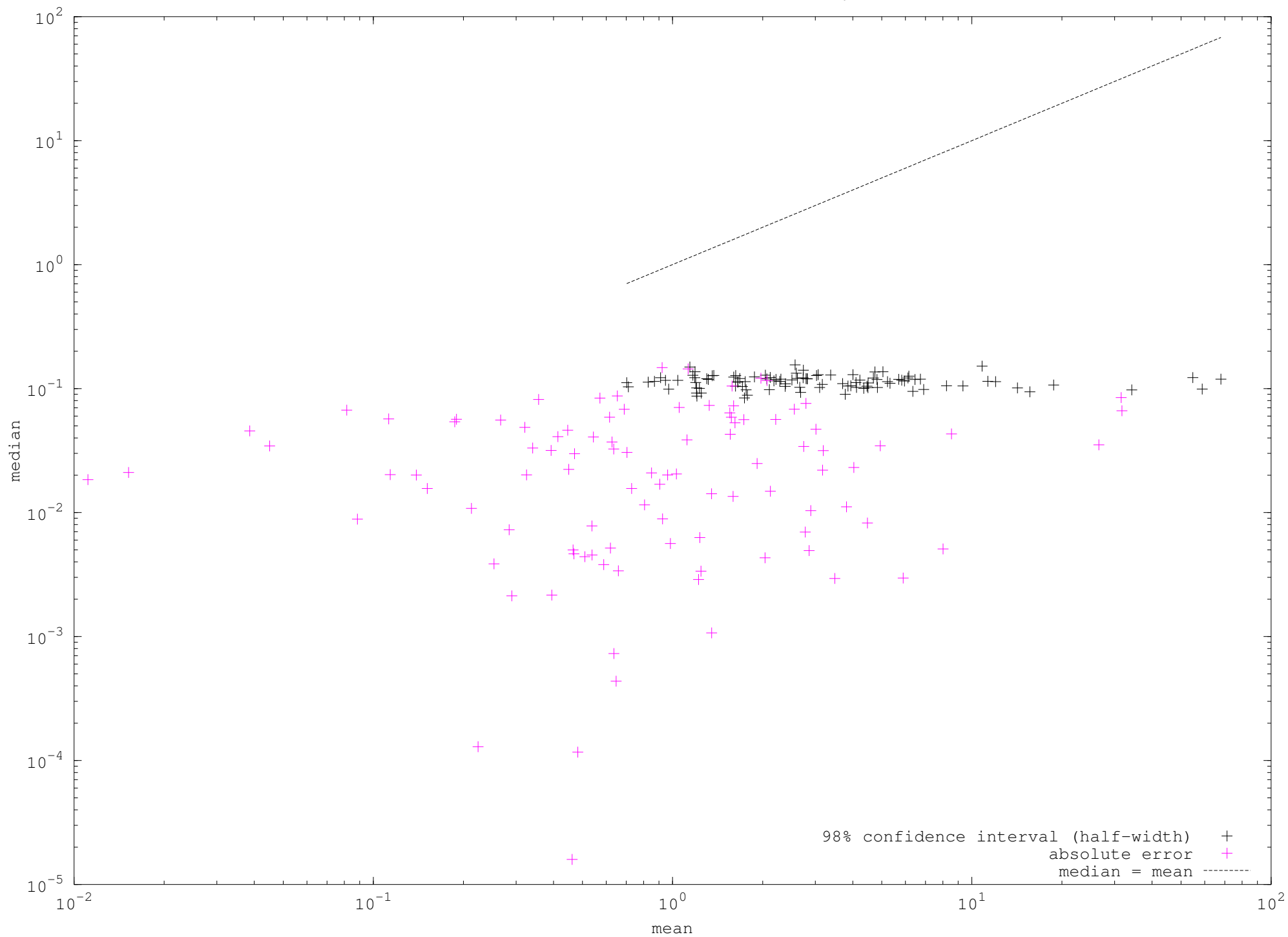
Bootstrap of sample mean and median for 100 datasets Npoints=1000, Cauchy distributed data, x_0=0 , \gamma=1
