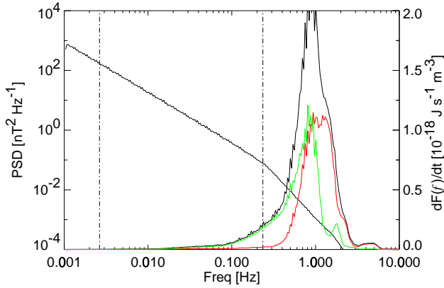
FIGURE 3. Synthetic power spectrum of Kinetic Alfvén waves (left-hand scale) and heating rate dF(f)/dt as a function of frequency. The total heating rate, which is the sum over all of the 250 logarithmically-spaced frequency bins used, is 6.36 \times 10^{-17} \text{ J s}^{-1} \text{ m}^{-3} . Under the heating rate curve are the electron and proton contributions, at slightly lower and higher frequencies, respectively.
