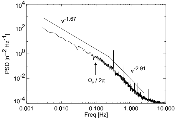
FIGURE 1. Trace of power spectral density matrix for hour 22UT, January 11, 1997, providing an example of a dissipation range power spectrum at 1 AU. For this period, B = 6.27 nT, \beta_p = 0.480 , \Theta_{BV} = 38.1^\circ , V_{SW} = 517 km s ^{-1} , and \Omega_p = 0.605 rad s ^{-1} (0.096 Hz). The spectral break frequency is computed to be 0.235 Hz. Spacecraft-generated spintones are seen at harmonics of 0.33 Hz and a noise signal exists above \sim 1 Hz.
