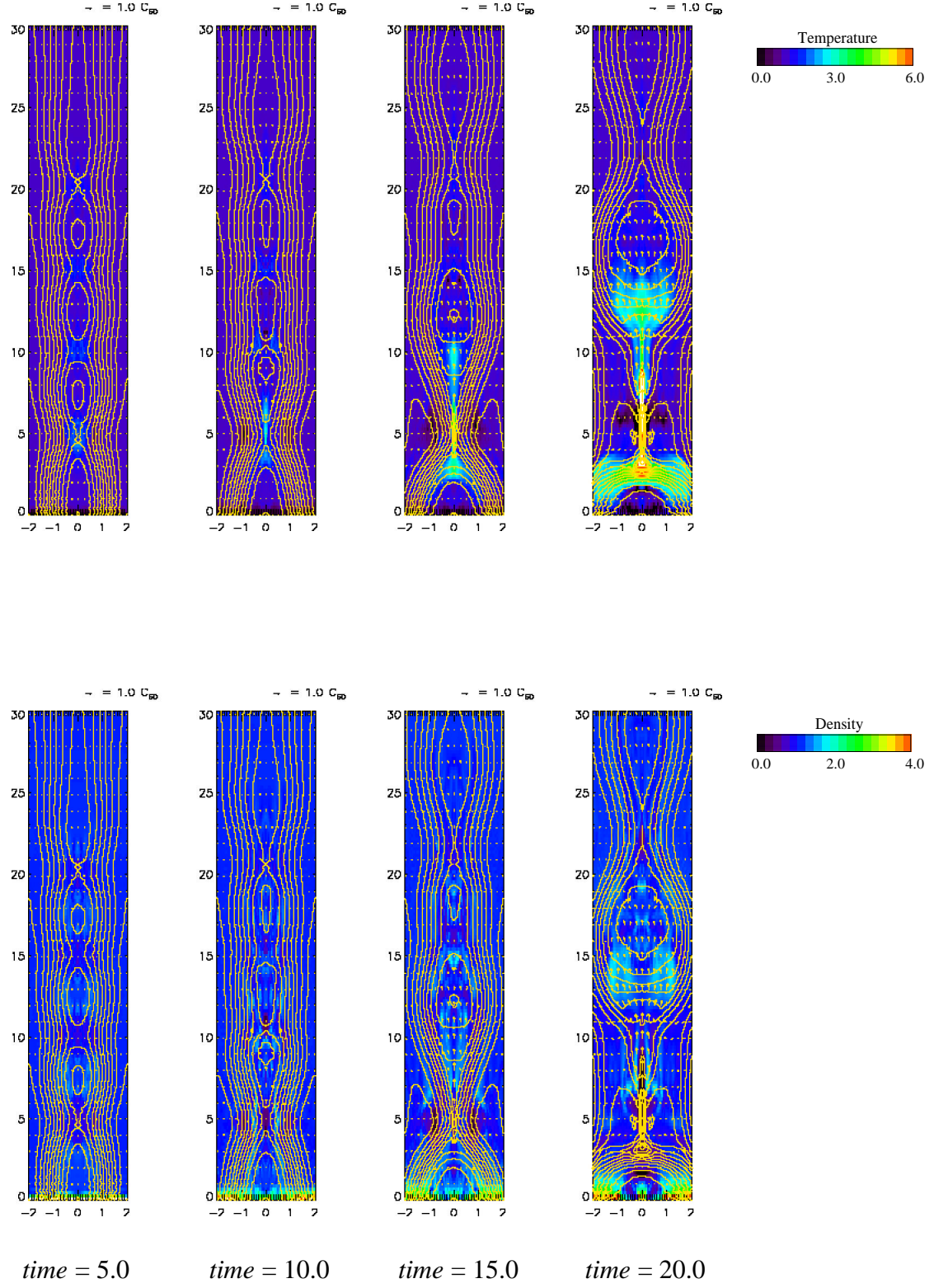
FIG. 3. 6a.—Evolution of model M. Top and bottom panels show the temperature and gas density maps, respectively. Contour lines and arrows represent the magnetic field lines and velocity field projected onto the (x, z) -plane. Elapsed times are t = 5, 10, 15 , and 20 from left to right.
