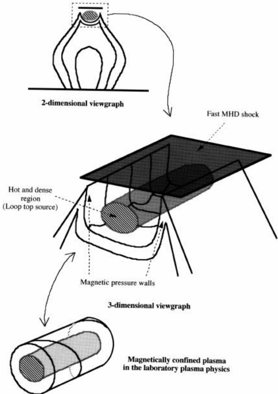
FIG.4. 4.—Schematic illustration of a loop-top region. From a 3-dimensional viewpoint, the loop-top source is no longer regarded as a circle-like source but a cylindrical one. Since the configuration of this is similar to that of a magnetically confined plasma in laboratories, we expect that the interchange instability can occur in the loop-top region in the same way as in the laboratory case.
