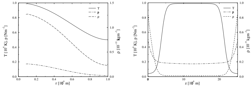
Figure 1. Radial and longitudinal variation of the initial temperature, pressure, and density profiles ( a = 10^6 m, L/a = 8\pi , B = 25 \times 10^{-4} T). left panel : at the loop top right panel : on axis.
