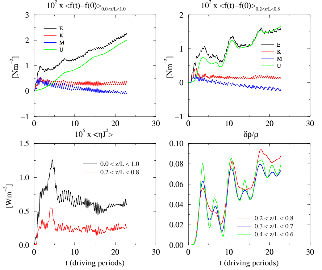
Figure 2. The evolution of volume averaged quantities for v_d = 23.5 km/s and P_{\text{driver}} = 41.1 s. Upper-left panel : Variation w.r.t. the initial state of the kinetic energy K , the magnetic energy M , the internal energy U , and the total energy (not including gravitational energy) E = K + M + U averaged over the whole loop structure. Upper-right panel : Same as the top left plot but averaged over the corona only. Lower-left panel : Ohmic dissipation rates. Lower-right panel : Relative density variations averaged over different parts of the corona.
