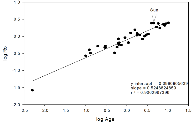
Fig. 5. The Rossby number (y-axis) versus age (x-axis) relationship as determined from our stellar sample. The Rossby number R_o is seen to increase with the star's age. Since the dynamo number N_d \sim 1/R_o^2 and a decrease in the dynamo number results in less efficient dynamo amplification of magnetic fields, it is theoretically expected that the level or amplitude of dynamo generated magnetic activity will decrease with age.
