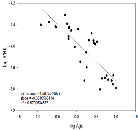
Fig. 7. Plotted here is the age dependence of chromospheric Ca H+K flux in our sample of stars. On the y-axis is a particular measure of the Ca H+K flux (attributed to magnetic activity) and on the x-axis is age. The data for the chromospheric emission has been compiled from various published sources related to the Mount Wilson project. The level of magnetically mediated chromospheric emission clearly decreases with age.
