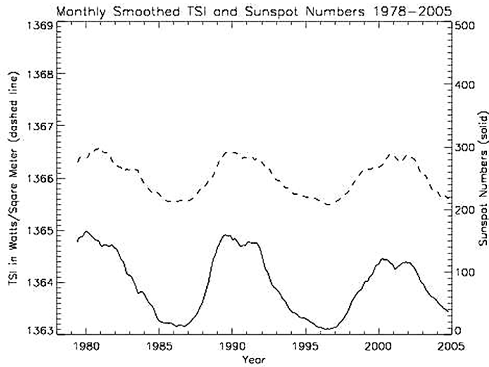
Fig. 1. The dashed curve shows the variation in TSI over time while the solid curve shows the solar cycle variation in the number of sunspots on the solar photosphere over the same period of time (monthly averages smoothed with a 13 month algorithm). The TSI variation is coupled to solar activity and varies in phase with it. The TSI data is courtesy of the World Radiation Center (Davos) and the sunspot data is courtesy of the Solar Influences Data Analysis Center (Belgium).
