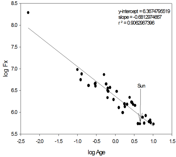
Fig. 8. The age (x-axis) dependence of the stellar coronal X-ray flux (y-axis) is shown here. The stellar X-ray flux has been determined from various published sources utilizing data from ROSAT, XMM-Newton, and other X-ray surveys. The stellar coronal X-ray emission is seen to decrease with age; the dependency is more pronounced and tighter than that for Ca H+K emission, indicating that X-rays may be a more useful diagnostic for such investigations.
