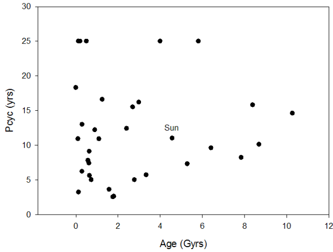
Fig. 6. The magnetic activity period (y-axis) versus age (x-axis) relationship in a subset of our stellar sample for which period measurements exist. No statistically significant trend is recovered in this sample.
