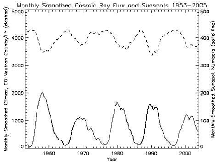
Fig. 2. The variation in the cosmic ray (neutron) flux (dashed line) and sunspot numbers (solid line) as observed over the last half-century. The anti-correlation between the two is clear. The smoothing algorithm is the same as in Figure 1. The cosmic ray data is courtesy the CLIMAX Neutron Monitor (Colorado).
