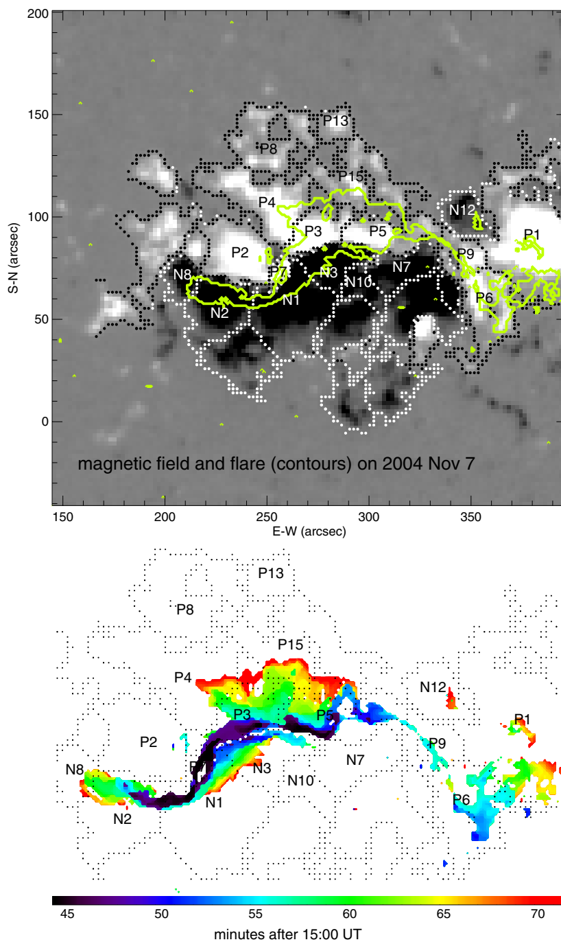
Fig. 2.— Top: photospheric magnetogram by MDI superimposed with the contours of flare areas at the maximum of the flare. “P” and “N” denote positive and negative magnetic cells, respectively. Bottom: temporal and spatial evolution of the flare superimposed on partitioned magnetogram. Time is indicated by the color code. Specifically, the number below the color bar indicates that at the time (minutes after 15:00 UT) indicated by the number, the flare ribbons expand to the areas shaded in the color above this number. For example, at 55 minutes after 15:00 UT, the flare ribbons expand to the areas shaded in light blue.
