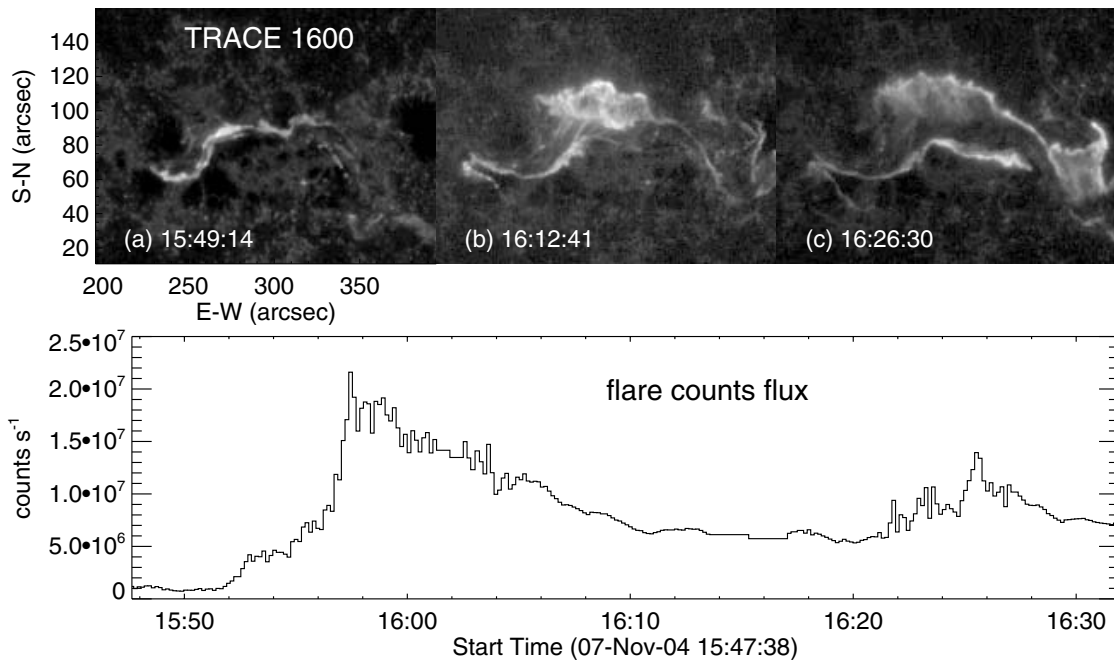
Fig. 1.— Top: snapshots of the X2.0 flare observed by TRACE 1600 Å on 2004 November 7. Bottom: the light curve of the count rates of the flare at 1600 Å (same as Figure 7 in Longcope et al. (2007).)
