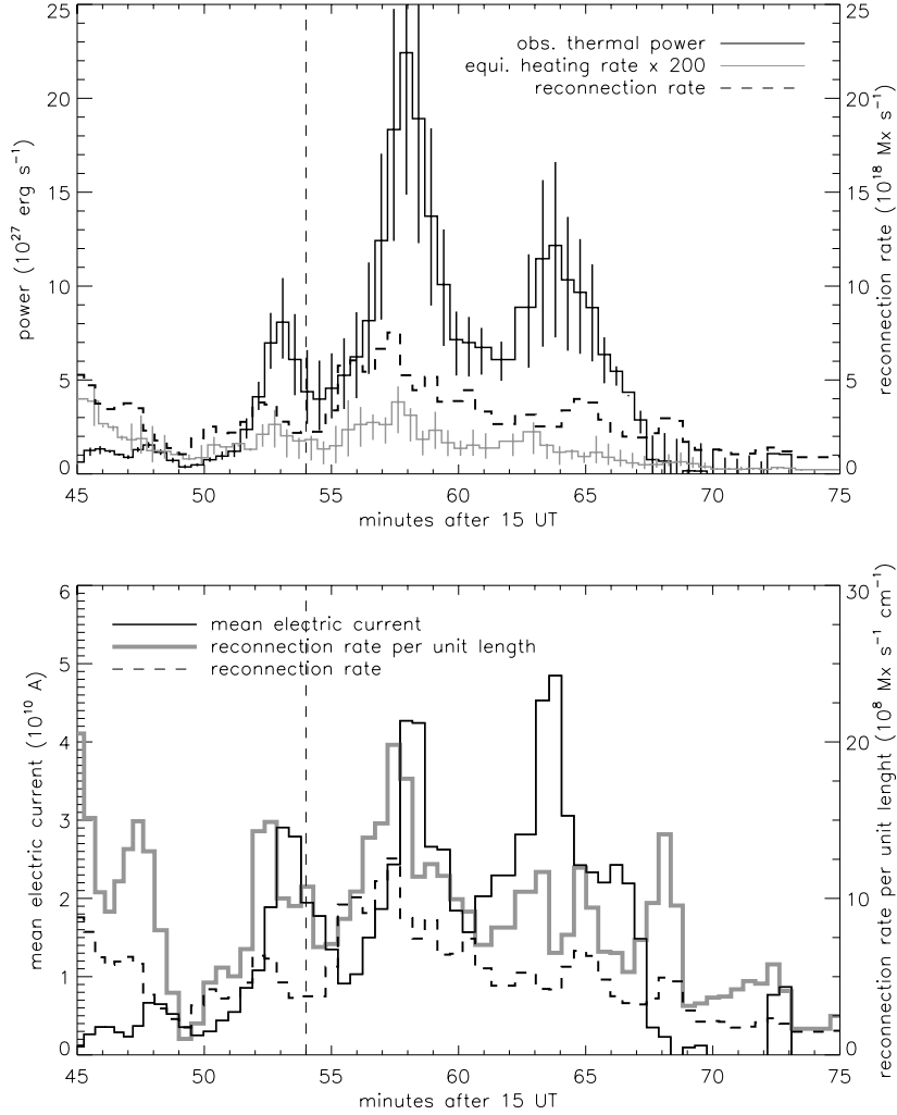
Fig. 9.— Estimates of reconnection energy release and reconnection electric current. Top: observed thermal energy release rate estimated from GOES diagnostics and morphological evolution of the flare (dark solid line) and estimated equilibrium heating rate from the scaling law (grey solid line). Vertical bars indicate the range of the estimates. The dashed curve shows the total reconnection rate. Bottom: mean electric current (dark solid line), reconnection rate per unit length (grey solid line), and total reconnection rate normalized to arbitrary units (dashed line). In both panels, the vertical dashed bar at 54 min indicates the division between two major stages of the flare.
