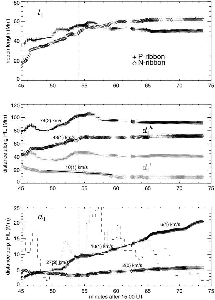
Fig. 4.— Global evolution of flare ribbons with respect to the PIL. Top: the total length l_{\parallel} of flare ribbons along the PIL. Middle: the distances of the “head” ( d_{\parallel}^h , dark symbols) and “tail” ( d_{\parallel}^t , grey symbols) points of the ribbon front along the PIL. Bottom: The mean distance d_{\perp} of the ribbon front perpendicular to the PIL. In all panels, the vertical dashed bar at 54 min indicates the division between two major stages of reconnection. In the bottom panel, the dashed curve indicates the total reconnection rate (the mean of the total reconnection rates derived from positive and negative polarities) arbitrarily normalized. The mean apparent speeds of flare ribbon elongation or expansion at different times are marked in the figures, and the numbers in the parentheses denote the \sigma in the speed derived from the least-squared fit.
