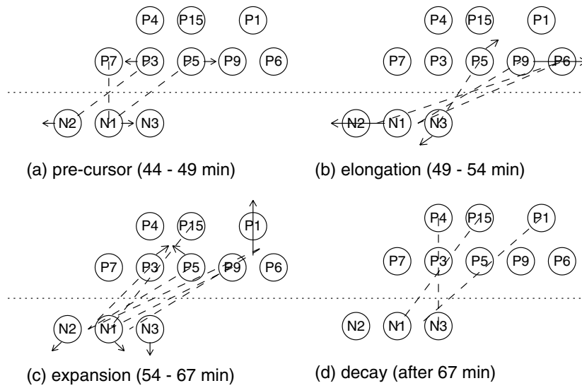
Fig. 8.— The sketch of connectivities between magnetic cells and evolution of cell brightening with respect to PIL during the flare. In each panel, circles give the relative positions of major magnetic cells that participate in reconnection and the dotted line marks the PIL. Dashed lines connect positive and negative cells that are reconnecting at a given episode as determined from the sequence analysis. Arrows give the direction of the spread of brightening in the cell with respect to the PIL.
