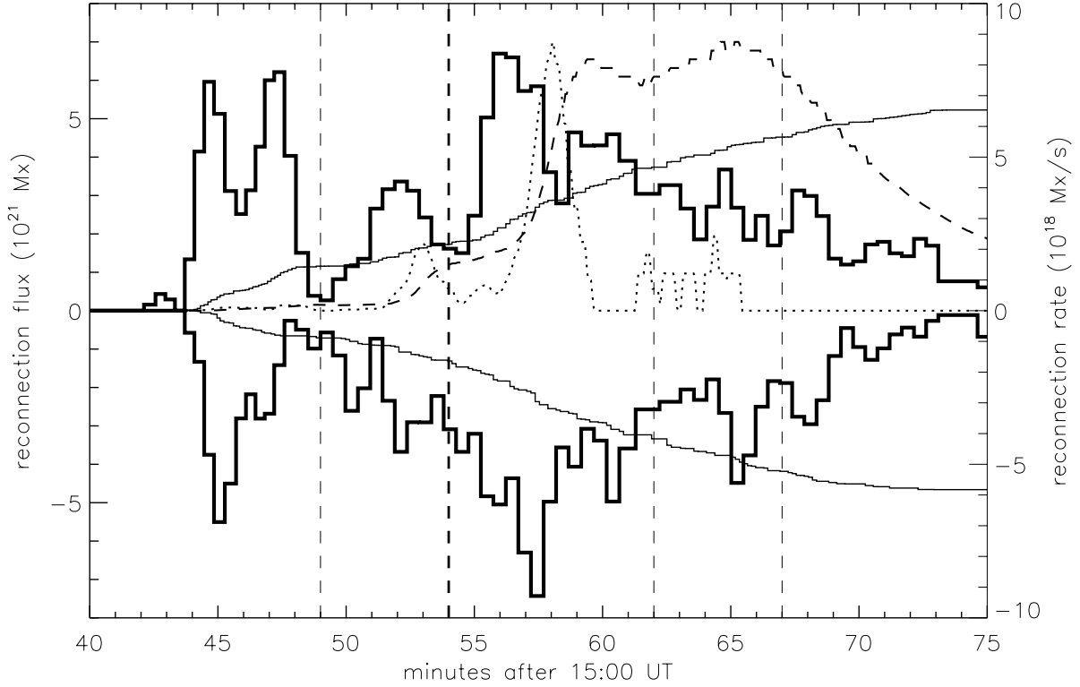
Fig. 3.— Time profiles of total reconnection flux in units of Mx (thin solid line) and reconnection rate in units of \text{Mx s}^{-1} (thick solid line) integrated in positive and negative polarities, respectively. Also shown are soft X-ray flux at 1 - 8\text{\AA} observed by GOES (thin dashed line) and its time derivative (thin dotted line), both normalized to arbitrary units. The maximum of the GOES X-ray flux at 1 - 8\text{\AA} is 6.6 \times 10^{-5} \text{ W m}^{-2} . The vertical dashed bars indicate five episodes of magnetic reconnection: 44 - 49, 49 - 54, 54 - 62, 62 - 67, 67 - 75 min after 15:00 UT. The thick dashed vertical bar at 54 min indicates the division of two major stages.
