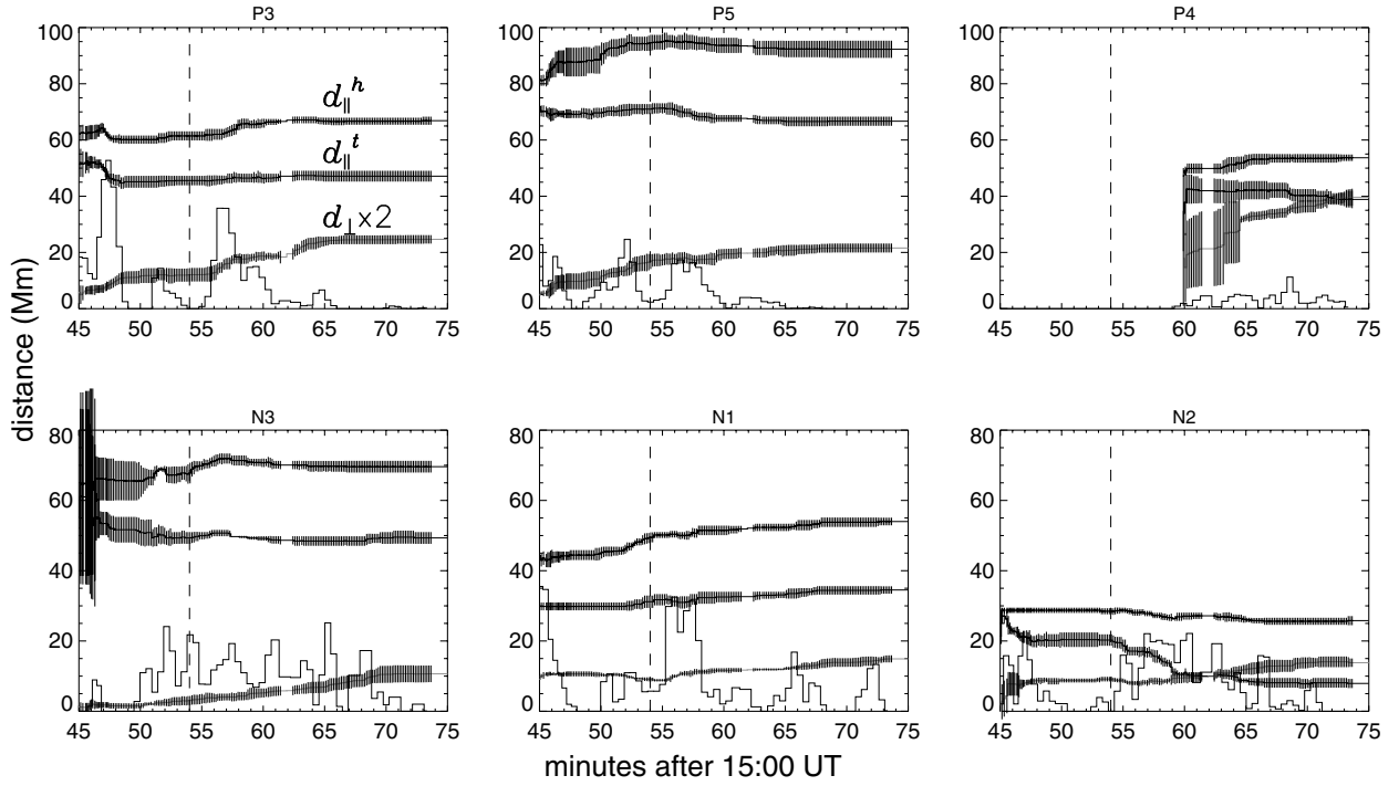
Fig. 5.— Spatially resolved evolution of flare brightenings in magnetic cells. In each panel, the three curves from the top to the bottom show measurements (in units of Mm) of d_{\parallel}^h , d_{\parallel}^t , and d_{\perp} , respectively, of the ribbon front in a major reconnection cell. Note that d_{\perp} is magnified by a factor of 2 for clarity. The vertical bars on the curve indicate the measurement uncertainty. In each panel, the thin solid curve shows the reconnection rate in the cell in units of 10^{17} \text{ Mx s}^{-1} .
