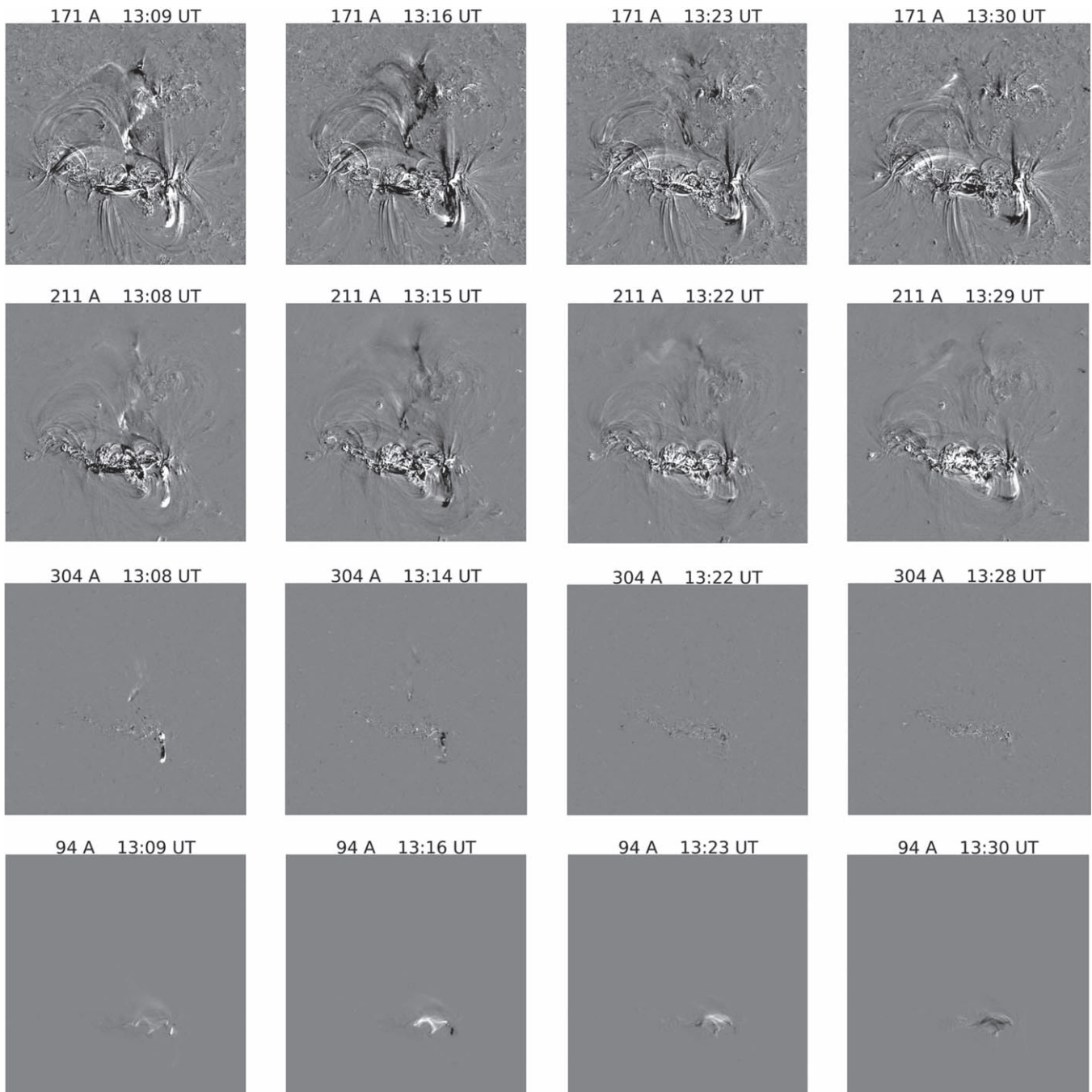
Figure 3. Absolute difference images of SDO/AIA centered on active region 12671 (see arrow 7 in Figure 2), which was near disk center and 10^\circ north latitude at the time of the eclipse. Each frame shows the change over a \approx 7 minute period. From top to bottom, the rows show emission changes from 17.1 nm (Fe IX), 21.1 nm (Fe XIV), 30.4 nm (He II), and 9.4 nm (Fe XVIII). These changes highlight a CME that occurred almost simultaneously with other eruptive events near the limb of the corona (see Figure 2).
