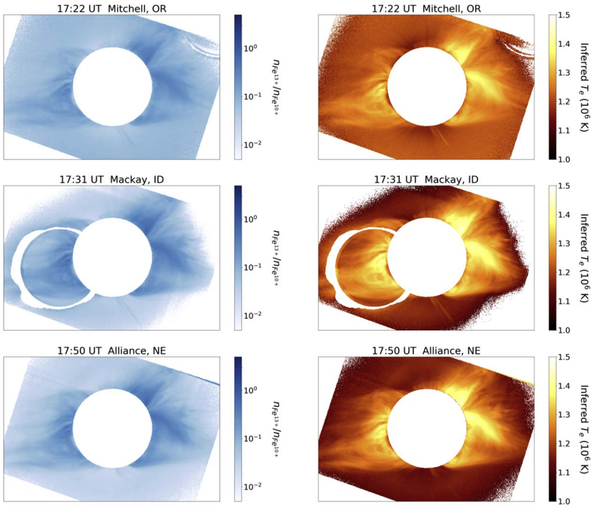
Figure 10. Left: Density ratio of Fe 13^+ to Fe 10^+ as calculated using Equation (9) (see Section 3.2.3) from the observations of Fe XI and Fe XIV made at three separate sites. Right: Inferred electron temperature ( T_e ) from the relative density measurements that were fed through the temperature function shown in Figure 9. The white ring in the middle panels indicates the location of a ghost image as in Figure 5.
