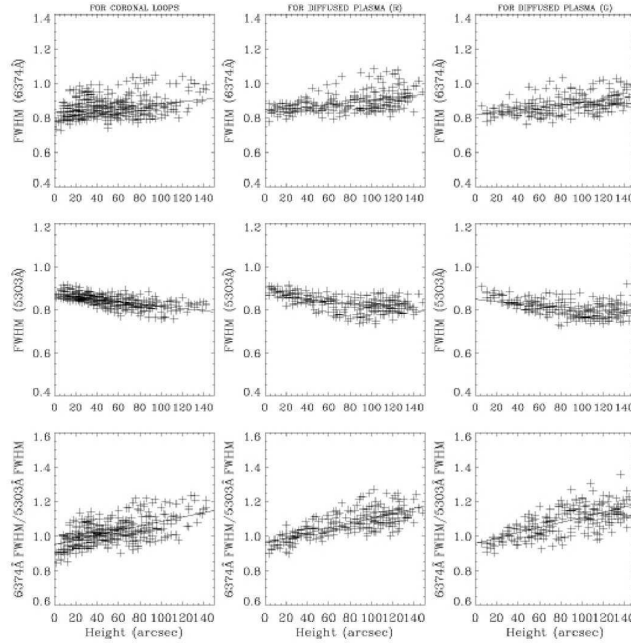
Figure 5. The variations in line widths of 6374 and 5303 Å lines with height above the limb in the coronal loop and the diffused plasma around the coronal loops.
