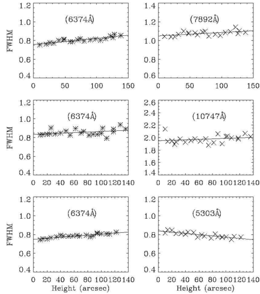
Figure 3. Variation of line widths with height above the limb in coronal loops observed in the 6374, 7892, 10747 and 5303 Å emission lines.
