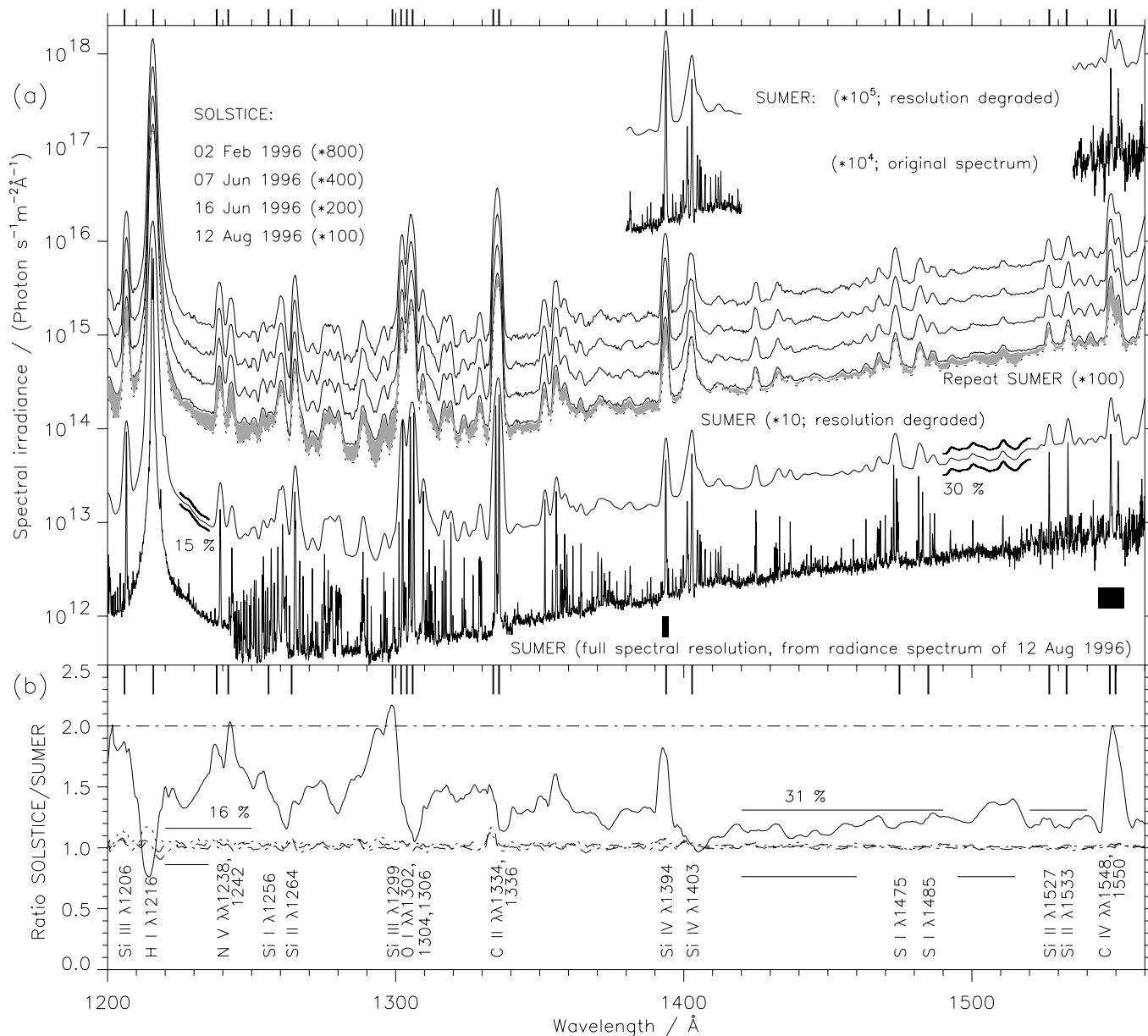
Fig. 1. a Spectra of SOLSTICE and SUMER in the wavelength range from 1200 Å to 1560 Å. The modified high-resolution radiance spectrum of SUMER is shown at the bottom multiplied by the solid angle of the Sun from 1 AU. The spectral resolution was then degraded to match that of SOLSTICE as shown in the next graph, after multiplication by 10 for display purposes. Near 1230 Å and 1500 Å the SUMER uncertainty margins ( 1\sigma ) are plotted as well. It is important to note that only the instrumental effects (including the count statistics) are taken into account, but not the solar variations. Four SOLSTICE irradiance spectra are shown over a period of approximately six months. In parallel to the SOLSTICE spectrum of 12 August 1996, the SUMER spectrum multiplied by 100 is repeated and the difference shaded in gray. The original SUMER spectrum and its low-resolution version are shown in the upper portion of panel a around those wavelength ranges where the spectrum below had been modified (as indicated by black bars). b The ratio SOLSTICE/SUMER is plotted for 12 August 1996 (solid line). Note that most of the wavelength range is dominated by emission lines, which influence this ratio by their different centre-to-limb variations. (For a discussion see Sect. 4.) The ratios of the various SOLSTICE spectra are shown as broken lines. Finally, the combined SOLSTICE/SUMER uncertainty margins (RMS) are indicated and some prominent emission lines are identified.
