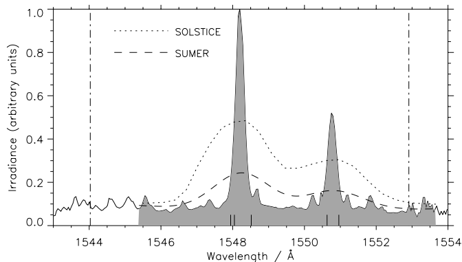
Fig. 2. Details of the wavelength range near the C IV lines are shown as high (solid line) and low resolution spectra (SOLSTICE: dotted line; SUMER: dashed line; not corrected for limb brightening). The irradiances are plotted in arbitrary units, but all three curves to the same scale. The shaded portion of the high-resolution spectrum has been used to determine the Si I line contribution in Table 3. The dashed-dotted lines mark the wavelength range in which the original spectrum in Fig. 1 has been substituted by the March 1999 data. The marks on the wavelength axis indicate those Si I lines which are very near the C IV lines.
