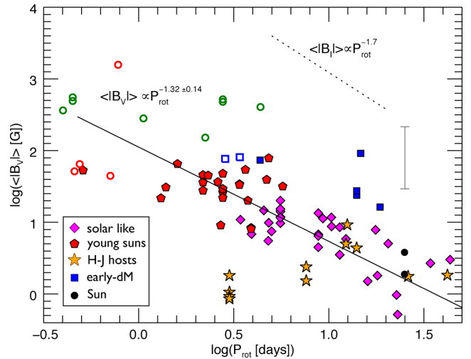
Figure 3. Correlation between the average large-scale field strength derived from the ZDI technique \langle |B_V| \rangle and rotation period P_{\text{rot}} , for the non-accreting stars in our sample. Our data support the presence of a linear-type dynamo for the large-scale field (i.e. \langle |B_V| \rangle \propto \Omega_* \propto P_{\text{rot}}^{-1} ) within 3\sigma , although a large scatter exists. The open symbols (not considered in the fit) are saturated M dwarf stars without age estimates: blue squares for M_* \geq 0.4 M_\odot (early Ms), green circles for 0.2 < M_*/M_\odot < 0.4 (mid Ms) and red circles for M_* \leq 0.2 M_\odot (late Ms). The dotted line, at an arbitrary vertical offset, is indicative of the slope found from ZB measurements between \langle |B_V| \rangle and P_{\text{rot}} (Saar 1996).
