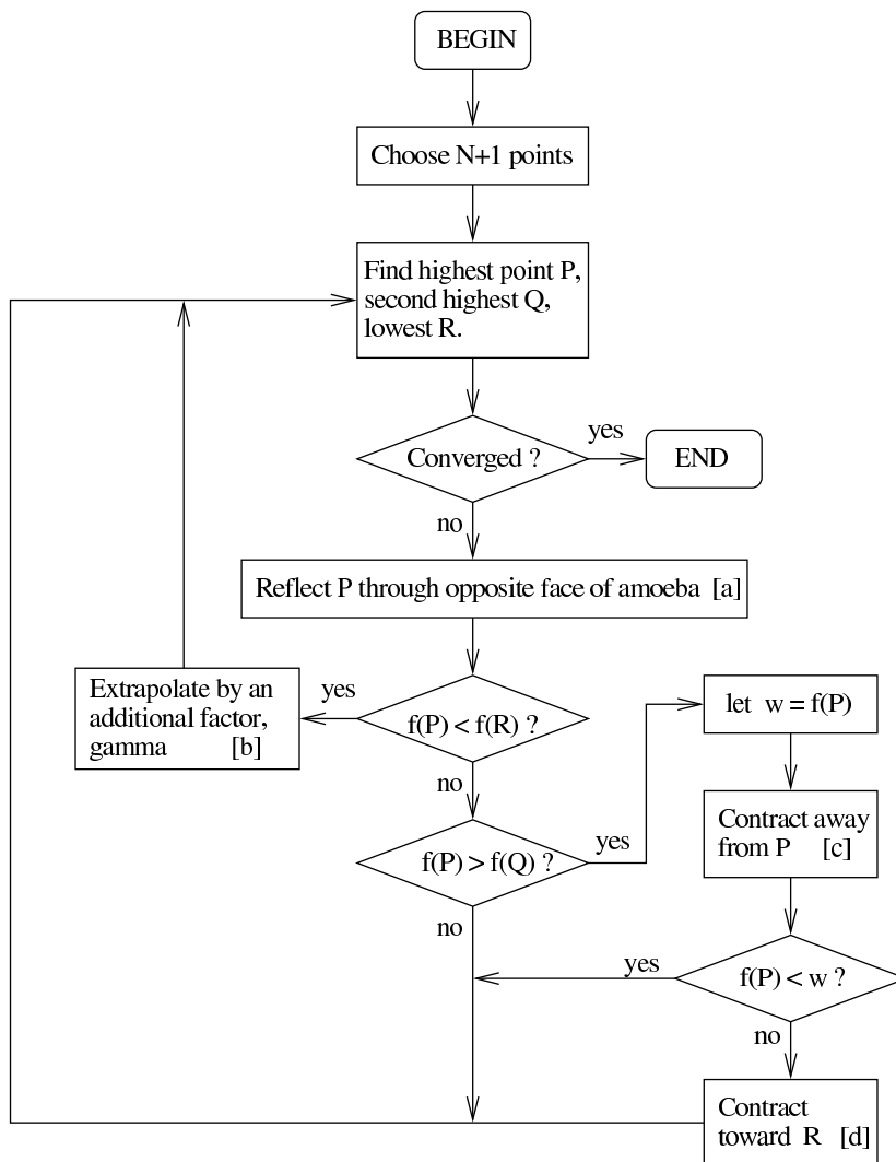
Fig. 2. Amoeba flowchart.
