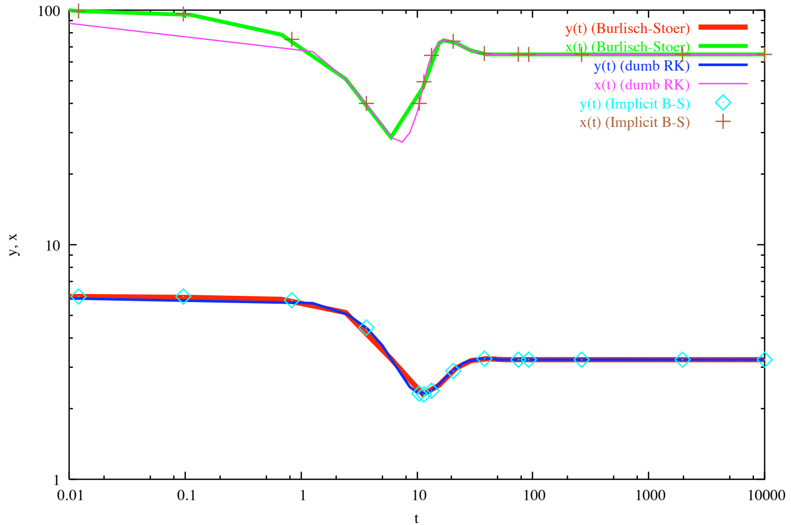
stiff equations
