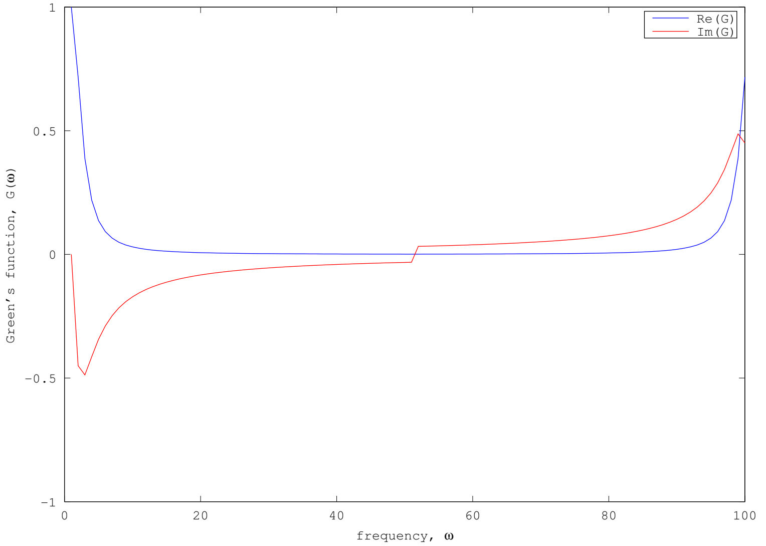
Green's Function for Lowpass Filter, RC = 1 \mu s
