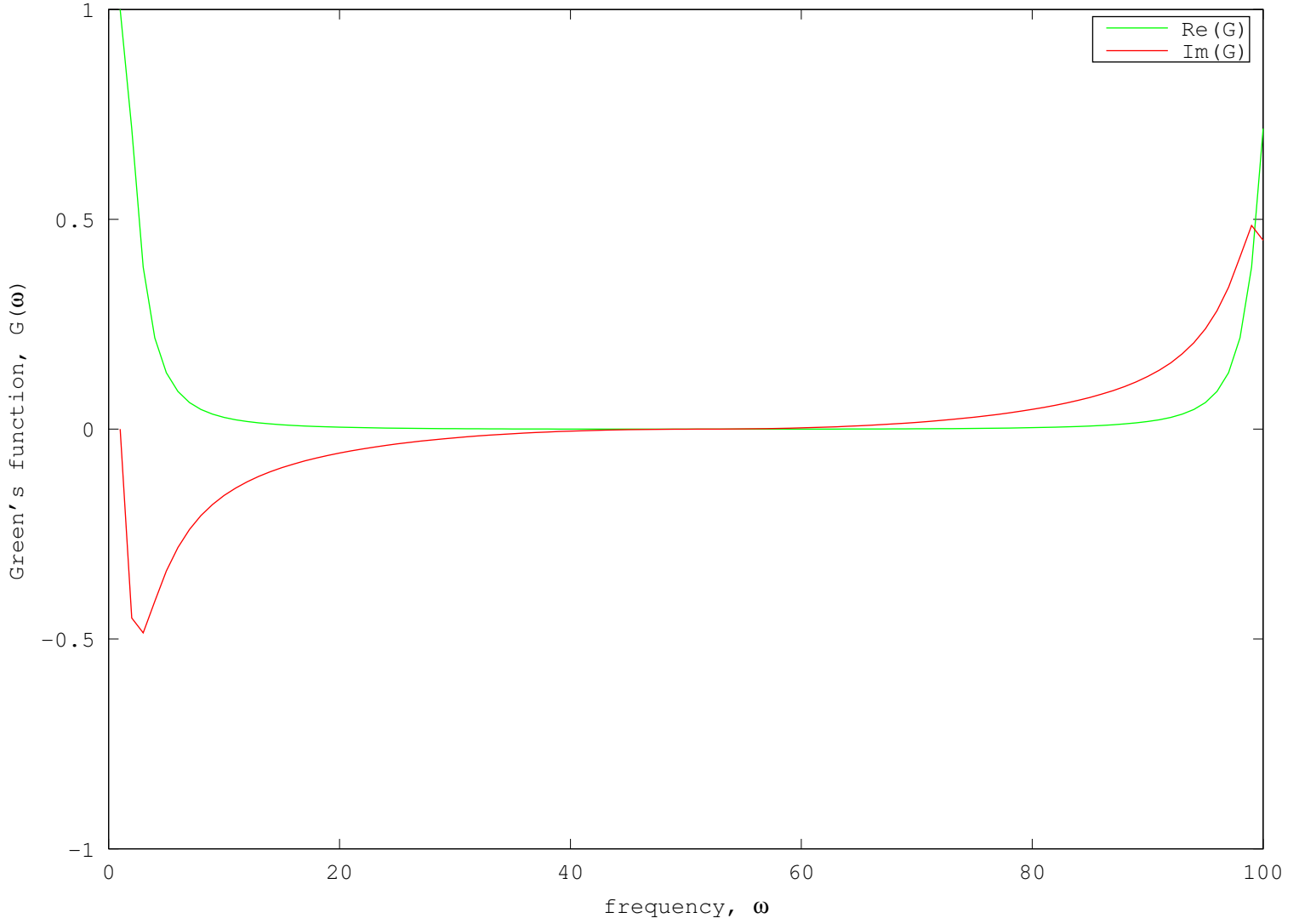
Anti-Aliased Green's Function for Lowpass Filter, RC = 1 \mu s
