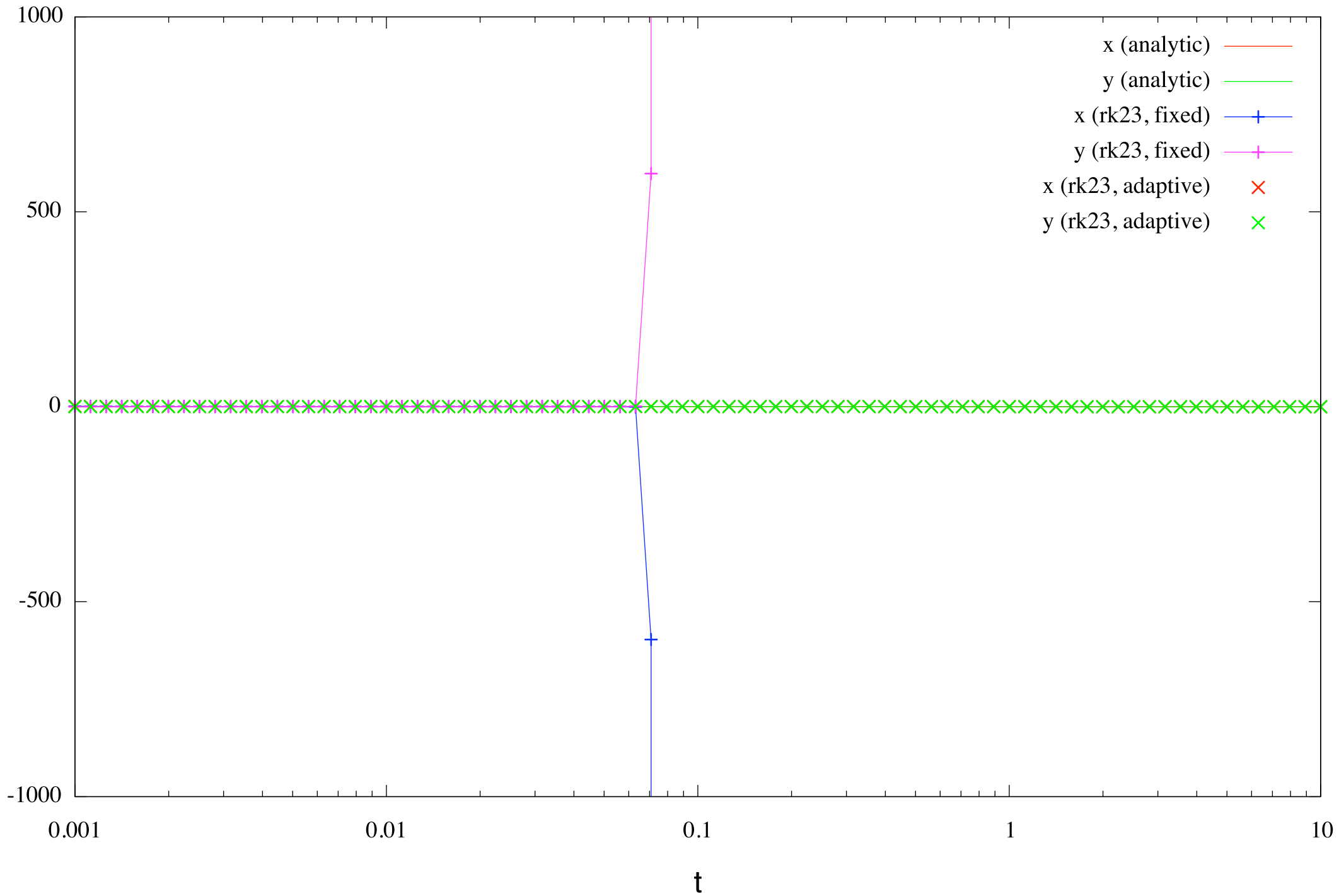
stiff_test1.m: CCK explicit solvers
