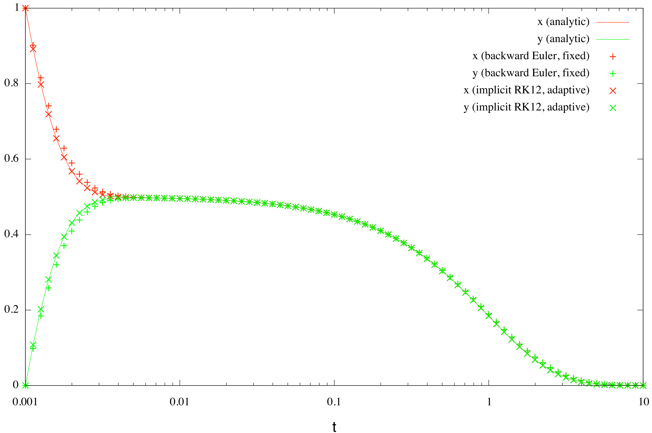
stiff_test1.m: CCK implicit solvers
