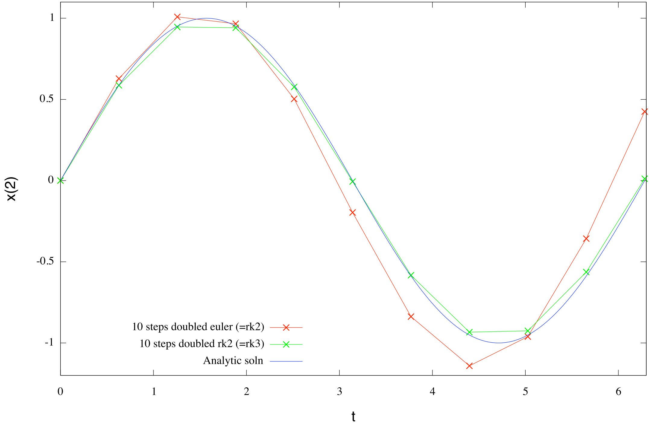
twostep_test1.m: test of step doubling
