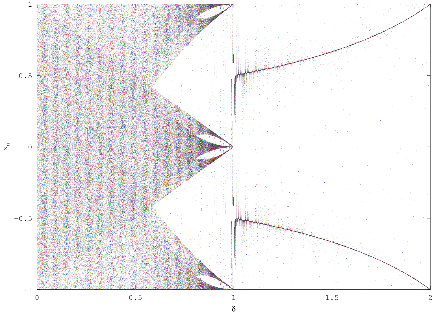
Card Shuffling: Bifurcation Diagram
